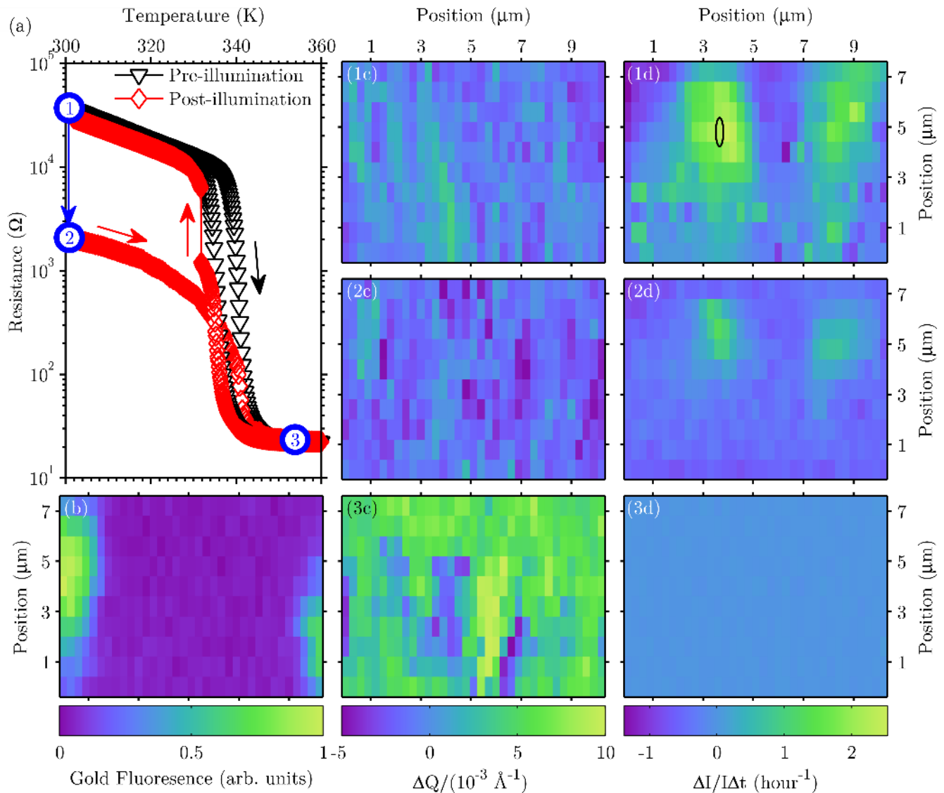
FIG. 2. (Color online). (a) The resistance is reduced by over one-order of magnitude at room temperature (point 1 to 2) by illuminating the device with x-rays at the indicated location in (1d) by the black ellipse. The resistance versus temperature hysteresis shows that the thermal component of the insulator-metal transition occurs at the same temperature for post-illumination (red diamonds) as no x-ray exposure (black down-pointing triangles). The original state is recovered by annealing the sample at 400 K and returning to room temperature. The device maps (b) to (d) are generated by scanning x-rays starting from the bottom-left corner proceeding in a series of horizontal lines. (b) Gold fluorescence intensity indicates the electrodes that define the device area. (c) Change in out-of-plane Bragg peak as compared to monoclinic phase and (d) normalized change in conductance induced by x-ray exposure for (1) 300 K and 40 k \Omega resistance before significant x-ray exposure in the monoclinic phase with \langle Q \rangle_M = 2.590 \text{ \AA}^{-1} and \langle \Delta I/I\Delta t \rangle_M = +0.3 \text{ h}^{-1} ; (2) 300 K and 2 k \Omega resistance after x-ray exposure with \langle Q \rangle_{PPC} = 2.589 \text{ \AA}^{-1} and \langle \Delta I/I\Delta t \rangle_{PPC} = -0.3 \text{ h}^{-1} ; (3) 354 K and 25 \Omega resistance in the tetragonal phase with \langle Q \rangle_R = 2.594 \text{ \AA}^{-1} and \langle \Delta I/I\Delta t \rangle_R = 0.0 \text{ h}^{-1} .
