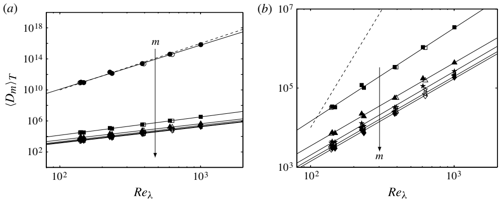
FIGURE 7. Scaling of \langle D_m \rangle_T and ratios as a function of Re_\lambda for forced stationary isotropic turbulence with resolutions up to 4096^3 : (a) D_m versus Re_\lambda for m = 1 – 6 , while (b) is a zoom of (a) to highlight the ordering of \langle D_m \rangle_T for m = 2 – 6 . In both parts the dashed lines correspond to Re_\lambda^6 .
