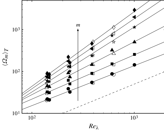
FIGURE 6. Scaling of \langle \Omega_m \rangle_T as a function of Re_\lambda for forced stationary isotropic turbulence with resolutions up to 4096^3 . Lines are for m = 1 (circles), m = 2 (squares), m = 3 (triangles), m = 4 (stars), m = 5 (left triangles) and m = 6 (diamonds). Open and closed symbols correspond to EP and FEK forcing, respectively. Dashed line is \sim Re_\lambda^6 (see the text). Note that for Re_\lambda \approx 650 at 4096^3 with FEK forcing, moments up to fourth order (instead of sixth) are available from our database.
