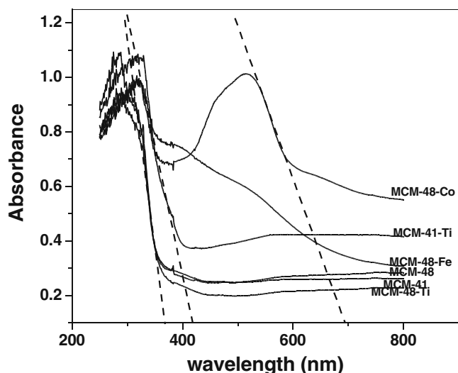
Figure 4. UV-vis spectra of the various catalysts.
