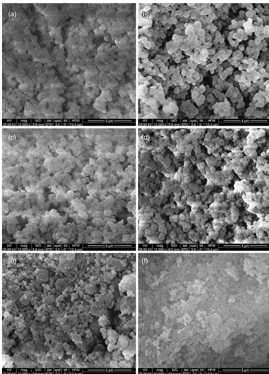
Figure 1. SEM images of the various catalysts. (a) MCM-41, (b) MCM-48, (c) MCM-41-Ti, (d) MCM-48-Ti, (e) MCM-41-Co, (f) MCM-48-Fe.
