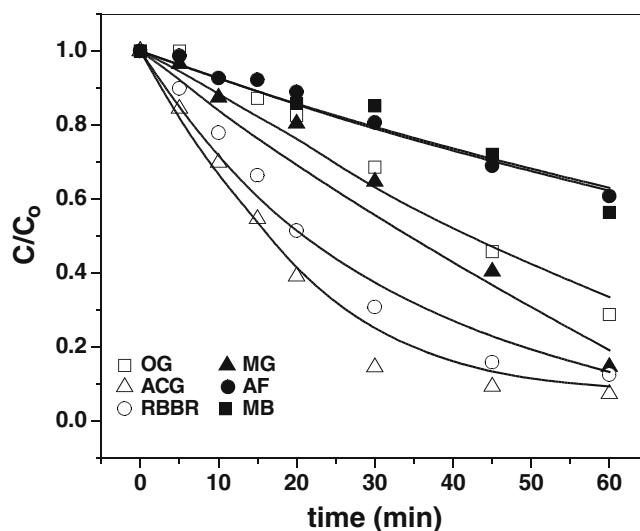
Figure 6. Variation of normalized concentration of different anionic and cationic dyes over MCM-48-Co.
