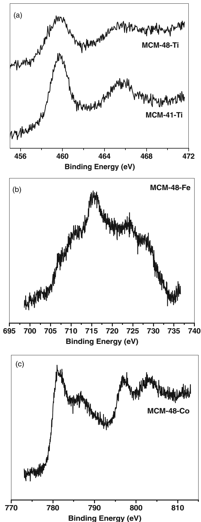
Figure 2. X-ray photoelectron spectra of (a) Ti2p, (b) Fe2p, (c) Co2p.
