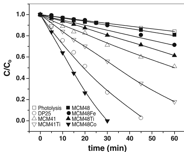
Figure 5. Variation of normalized concentration of IC with time over the different catalysts.
