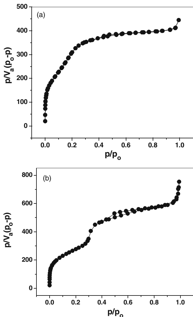
Figure 3. N_2 adsorption–desorption profile for (a) MCM-41, (b) MCM-48.
