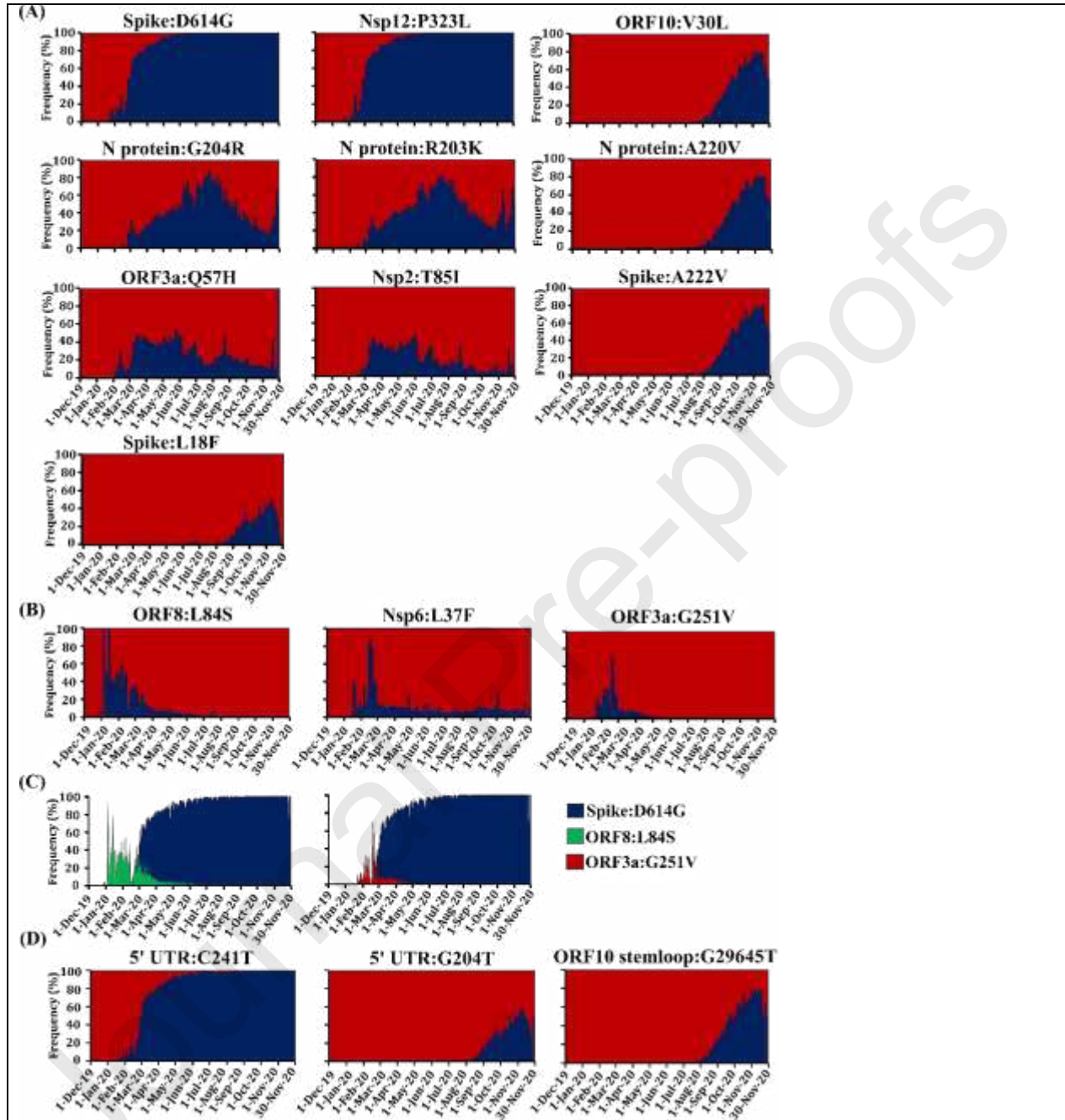
Figure 1: Month wise occurrence of key recurrent SARS-CoV-2 mutations. (A) Month wise occurrence of top 10 recurrent SARS-CoV-2 mutations. (A: Last column) Emergence of new highly recurrent (HR) mutations that occur after August 2020. Note that the emergence of N protein:A220V, ORF10 protein:V30L, Spike:A222V and Spike:L18F is seen only after July 2020. (B) Decrease in the percentage frequency of some of the mutations which were highly recurring before March 2020. Note that the occurrence of ORF8 protein:L84S and ORF3a protein:G251V is completely reduced after May 2020 and the occurrence of NSP6:L37F is reduced from HR to moderately recurrent (MR) after March 2020. (C) Diagram illustrating the rise (before Spike:D614G becomes dominant) and fall (after Spike:D614G takes over the wild type) of ORF8 protein:L84S and ORF3a protein:G251V. (D) Emergence of new mutations in non-coding region that occur at significantly high recurrence (HR). Note that 5'UTR:C241T mutation started occurring after Feb 2020 and 5'UTR:G204T and ORF10 stemloop:G29645T mutations started occurring after August 2020.
