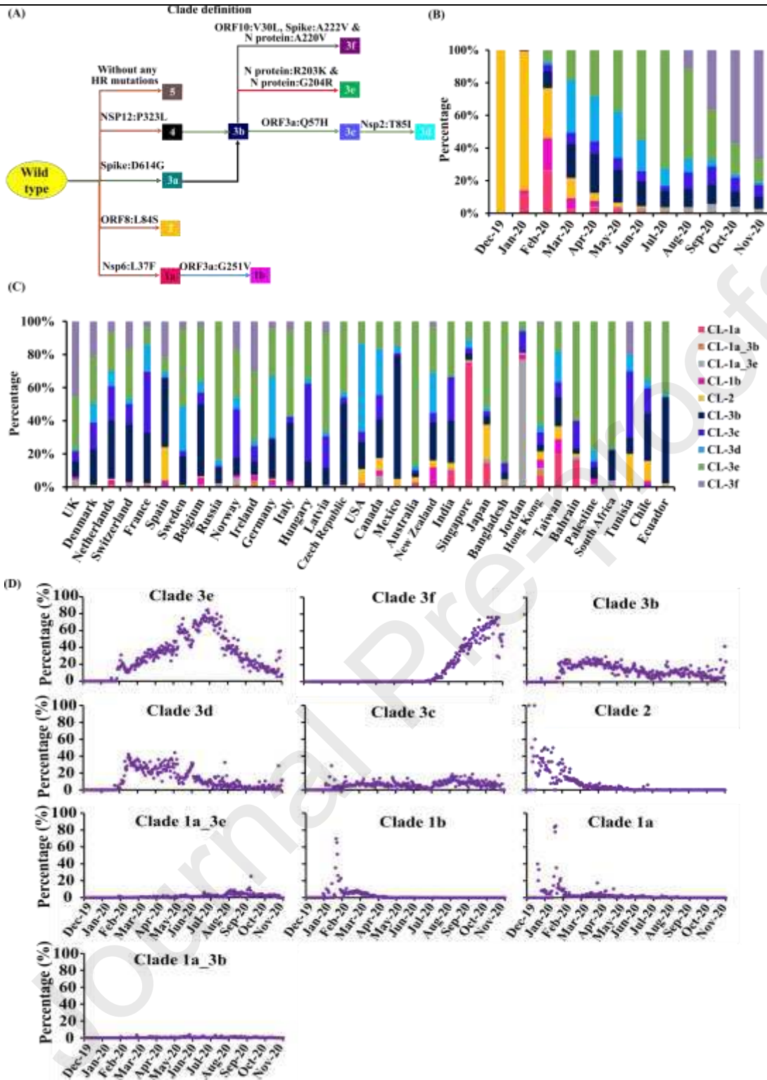
Figure 4: SARS-CoV-2 proteome clades dissemination. (A) SARS-CoV-2 proteome clade definition based on highly recurrent (HR) mutations. (B) Month wise and (C) country wise distribution of top 10 clades of SARS-CoV-2 and their mergers. (B) Note that CL-3e (light green color) is majorly distributed after March 2020 to August 2020, after that it started reducing and CL-3f (violet color) is majorly distributed after August 2020. (C) The CL-3f (violet color) is majorly distributed in European countries and CL-3e (light green color) is distributed in almost all the countries. (D) Month wise percentage occurrence of top 10 clades. Note the steady increase in clade 3f from August, 2020.
