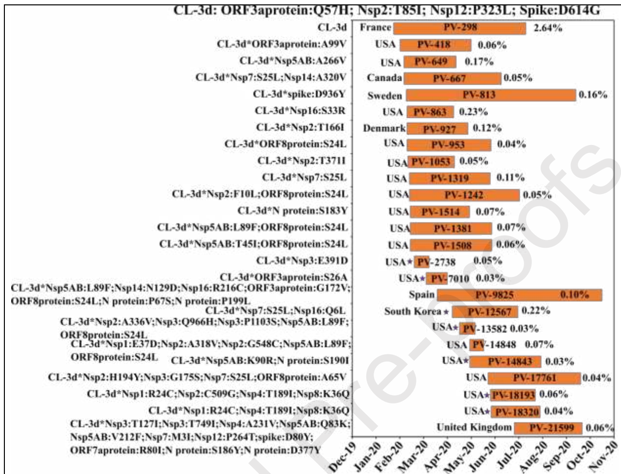
Figure 5: Month wise evolutionary dynamics of clade 3d (CL-3d) showing the divergence of the sub-clades from its ancestors. From the month (X-axis) of first emergence to the month of last appearance of a sub-clade in a particular country is represented by a bar. The variations in the amino acid sequence are given in the Y-axis. The country of first incidence is mentioned alongside the bar. The magenta colored star indicates that the sub-clade is country specific. PV number indicates the protein variant number of the particular sub-clade (see text for details). Note that only top 25 sub-clades are shown here.
