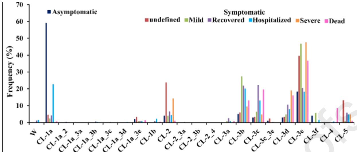
Figure 6: Histogram plot illustrating the distribution of the clades in SARS-CoV-2 patients. Note that the clade distribution is shown for asymptomatic, symptomatic (undefined), mild, recovered, hospitalized, severe and dead patients. Note that the CL-1a is highly distributed in asymptomatic patients and CL-1a, CL-2, CL-3b, CL-3c, CL-3d and CL-3e clades are distributed in all kind of patients.
