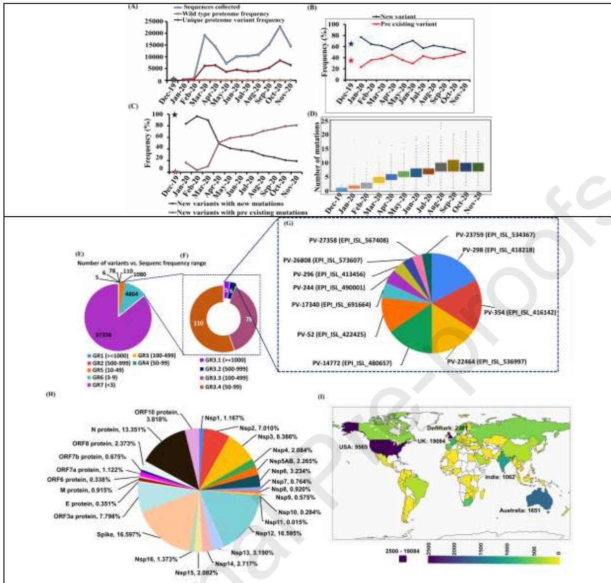
Figure 3: (A-D) Month wise summary of SARS-CoV-2 proteome variant distribution (Dec 2019 to Nov-2020) and (E-H) variant persistence. (A) Line plot illustrating the distribution of number of unique proteome variants (deep red color) from the total number of sequences collected (blue color) in that particular month. (B) Month wise sequence count (percentage frequency (%)) of appearance of new variants (colored dark blue) and preexisting variants (colored red). (C) Line plot illustrating the occurrence of new mutations in newly collected sequences (purple color) and without the occurrence of new mutations in newly collected sequences (pink color). (D) Box plot elucidating month wise occurrence of single amino acid mutations in SARS-CoV-2 sequences (Dec-2019 to Nov-2020). Note that the mutation average linearly increases every month in SARS-CoV-2 proteome. Due to the availability of less number of sequences in December 2019, it is indicated by “*”. (E-G) Relative percentage of occurrence of variants that are found in at least 3 (E) , 50 (F) and 500 (G) sequences. (H) Pie chart representing the protein wise variant distribution. (I) Country wise distribution of SARS-CoV2 variants. Note that the variant counts have been indicated for top 5 countries.
