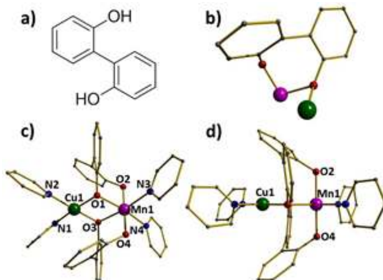
Figure 1. (a) The pro-ligand 2,2'-biphenol (LH 2 ) and (b) its coordination mode upon double deprotonation. Molecular structure of the heterobimetallic cation in 1 as viewed off-set (c) and perpendicular (d) to the Jahn-Teller compressed axis of the Mn(III) ion. Colour code: green (Cu), purple (Mn), red (O), blue (N) and grey (C). Hydrogen atoms and counter anions have been omitted for clarity.
