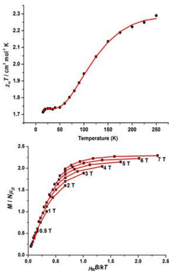
Figure 2. Upper panel: Plot of the \chi_M T product of 1 vs. T in the 250 - 5 K temperature range in an applied field of 0.1 T. The solid red line is the best-fit of the data with J = -33.4 \text{ cm}^{-1} as described in the text. Lower panel: Plot of reduced magnetisation of 1 in the 2.0 to 7.0 K temperature range and at the indicated field strengths. The solid red lines are the best-fit of the data with J fixed to -33.4 \text{ cm}^{-1} and D_{\text{Mn}} = +4.95 \text{ cm}^{-1} , as described in the text.
