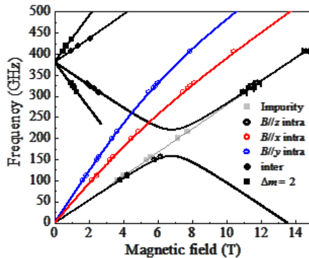
Figure 4. Plot of the frequency dependent EPR peak positions as a function of the applied magnetic field strength. The solid curves (same colour coding as the data) correspond to the simulations described in the main text. Note that the grey data points and the grey line correspond to an impurity signal with g = 2.003(2) .
