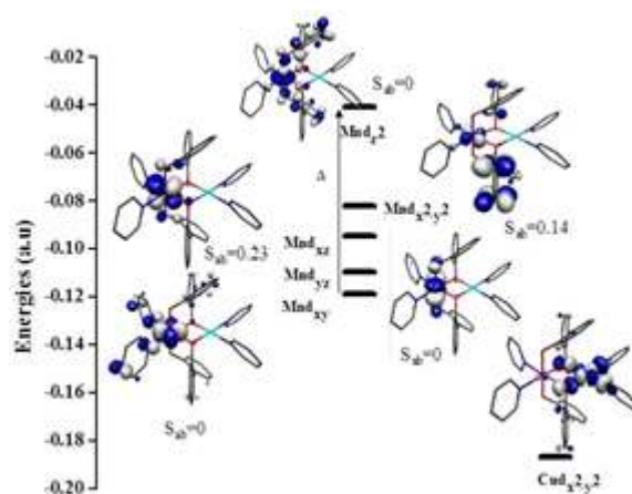
Figure 5. DFT calculated magnetic orbitals of Mn(III) and Cu(II) with computed S_{ab} (overlap integral) values. The isodensity surface represented corresponds to a value of 0.05 \text{ e}^-/\text{bohr}^3 .
