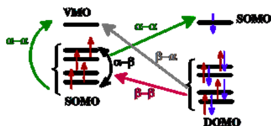
Figure 7. Schematic illustrating the different contribution to anisotropy in complex 1.
