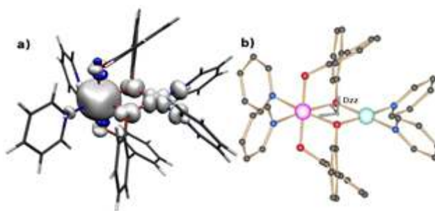
Figure 6. a) DFT computed spin density plot of 1 for the S = 2 state. The isodensity surface represented corresponds to a value of 0.005 e^-/\text{bohr}^3 . The white and blue regions indicate positive and negative spin populations, respectively. b) DFT calculated orientation of D -tensor in 1 . H-atoms have been omitted for clarity.
