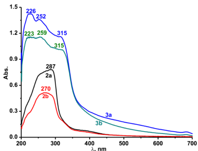
Figure 2. The solid state UV-vis spectra of 2a , 2b , 3a and 3b .
