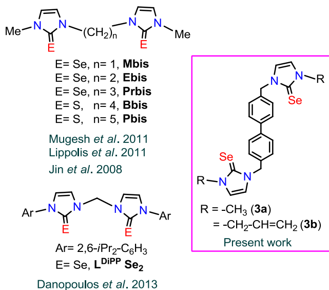
Chart 1. Known bis-imidazoline selenes.
