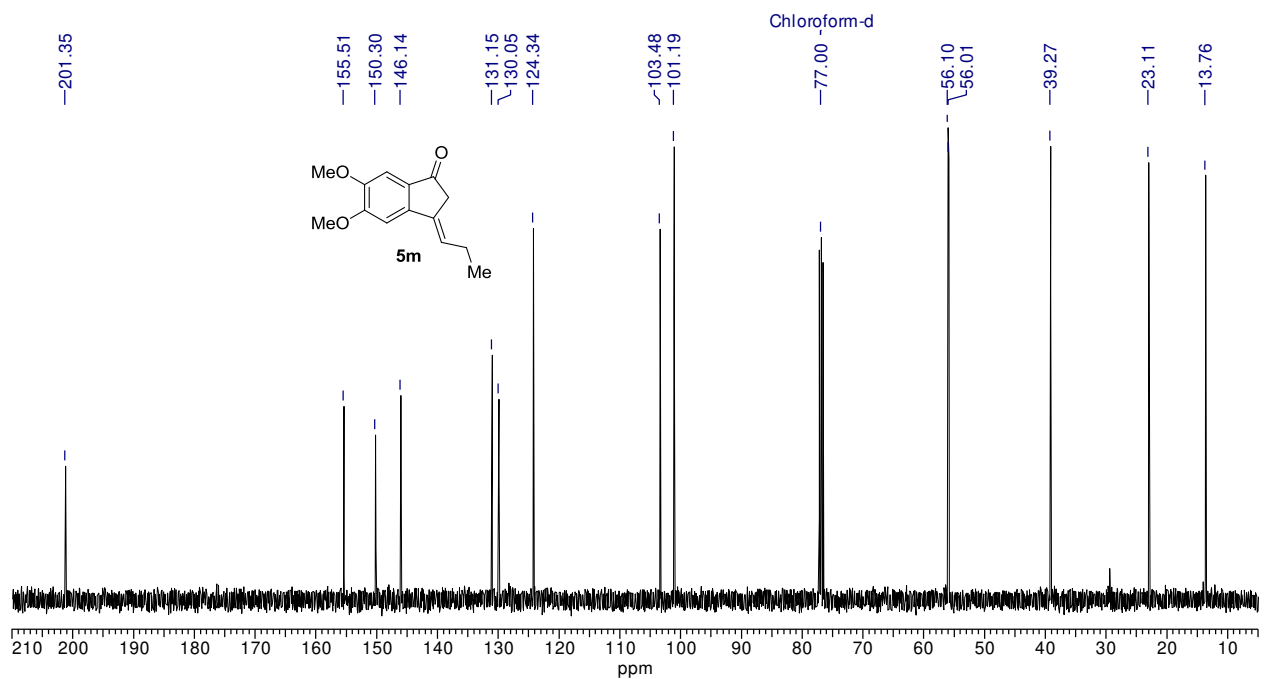
Figure II.4: 13 C-NMR (100 MHz) spectrum of 5m in CDCl 3
