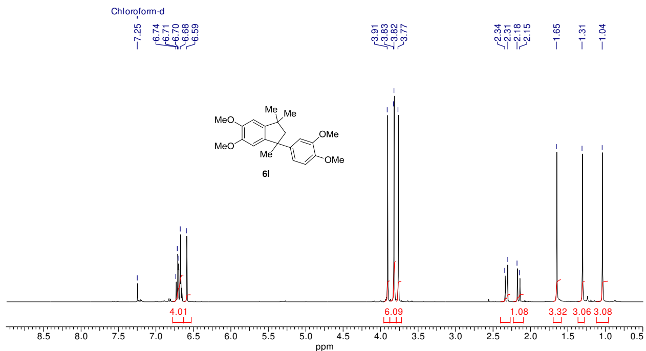
Figure III.10: ^1\text{H-NMR} (400 MHz) spectrum of 6l in \text{CDCl}_3 .
