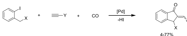
Scheme II.12
