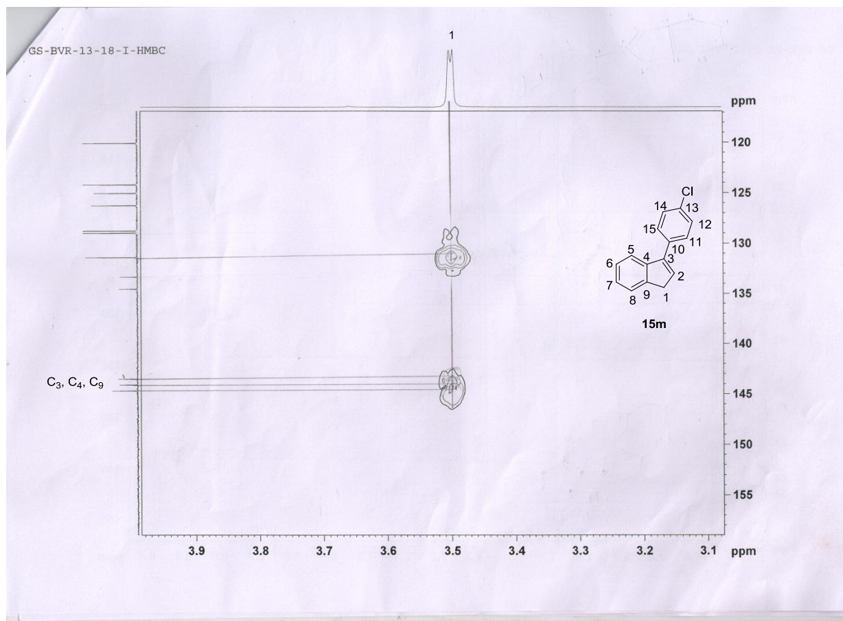
Figure II.21: HMBC-NMR (400 MHz) spectrum of 15m in CDCl 3
