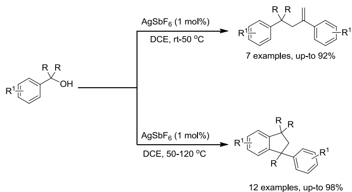
Scheme III.14
