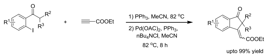
Scheme II.4
