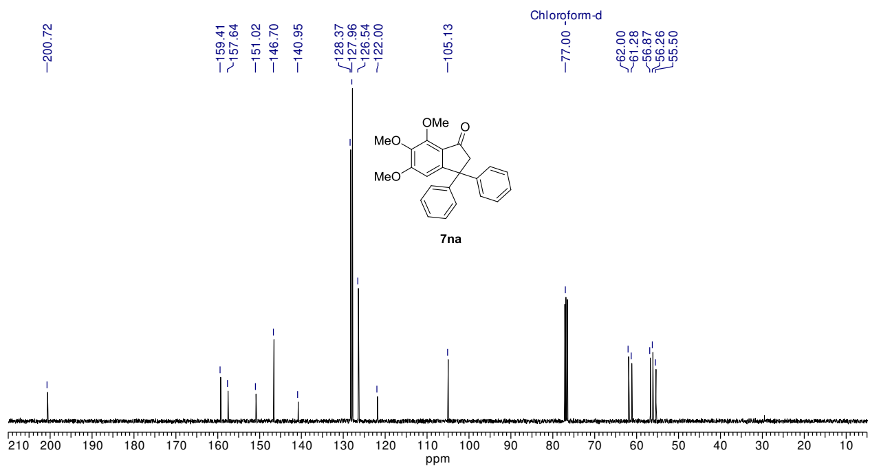
Figure I.15: ^{13}\text{C-NMR} (100 MHz) spectrum of 7na in \text{CDCl}_3
