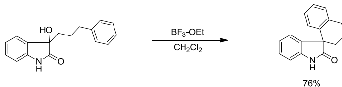
Scheme II.20
