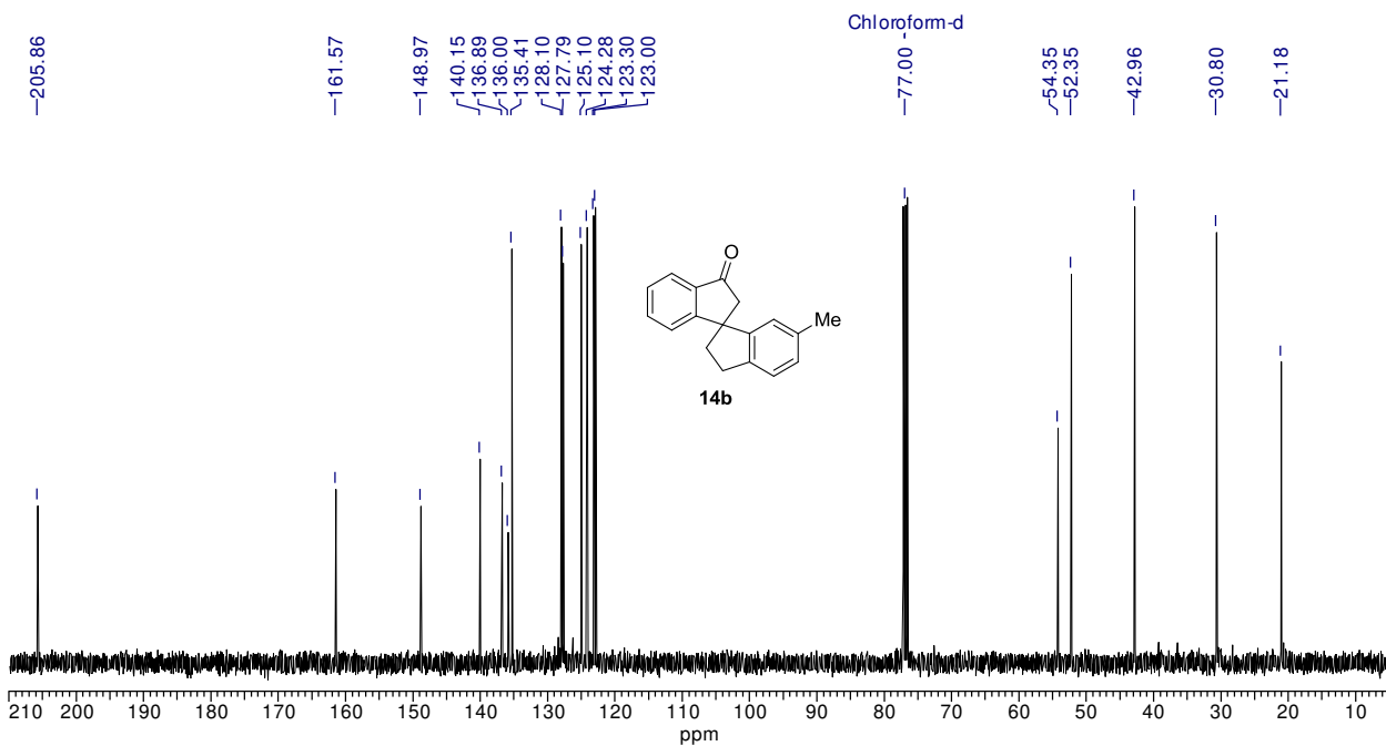
Figure II.28: ^{13}\text{C} -NMR (100 MHz) spectrum of 14b in \text{CDCl}_3
