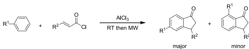
Scheme I.4
