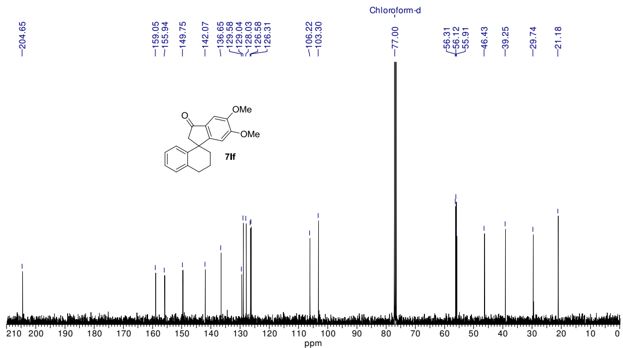
Figure I.19: ^{13}\text{C-NMR} (100 MHz) spectrum of 7lf in \text{CDCl}_3
