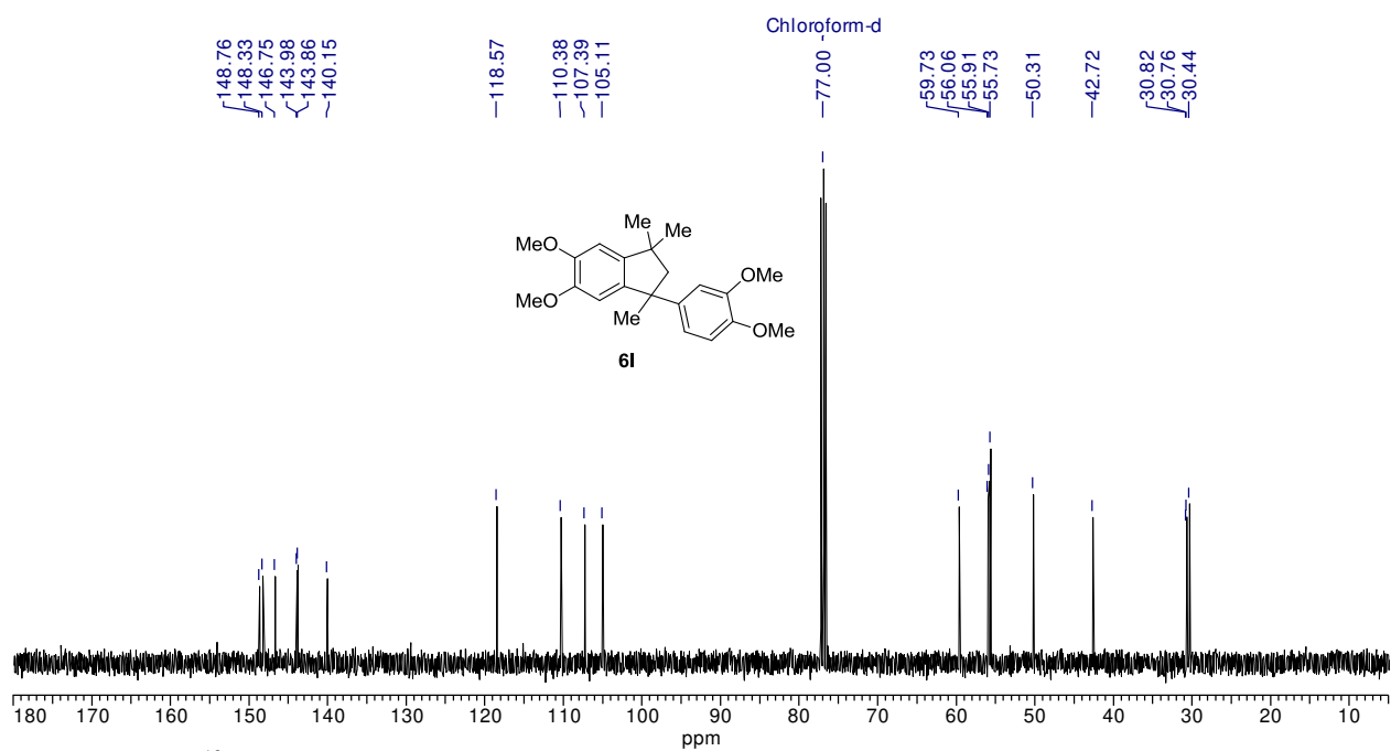
Figure III.11: ^{13}\text{C-NMR} (100 MHz) spectrum of 6l in \text{CDCl}_3 .
