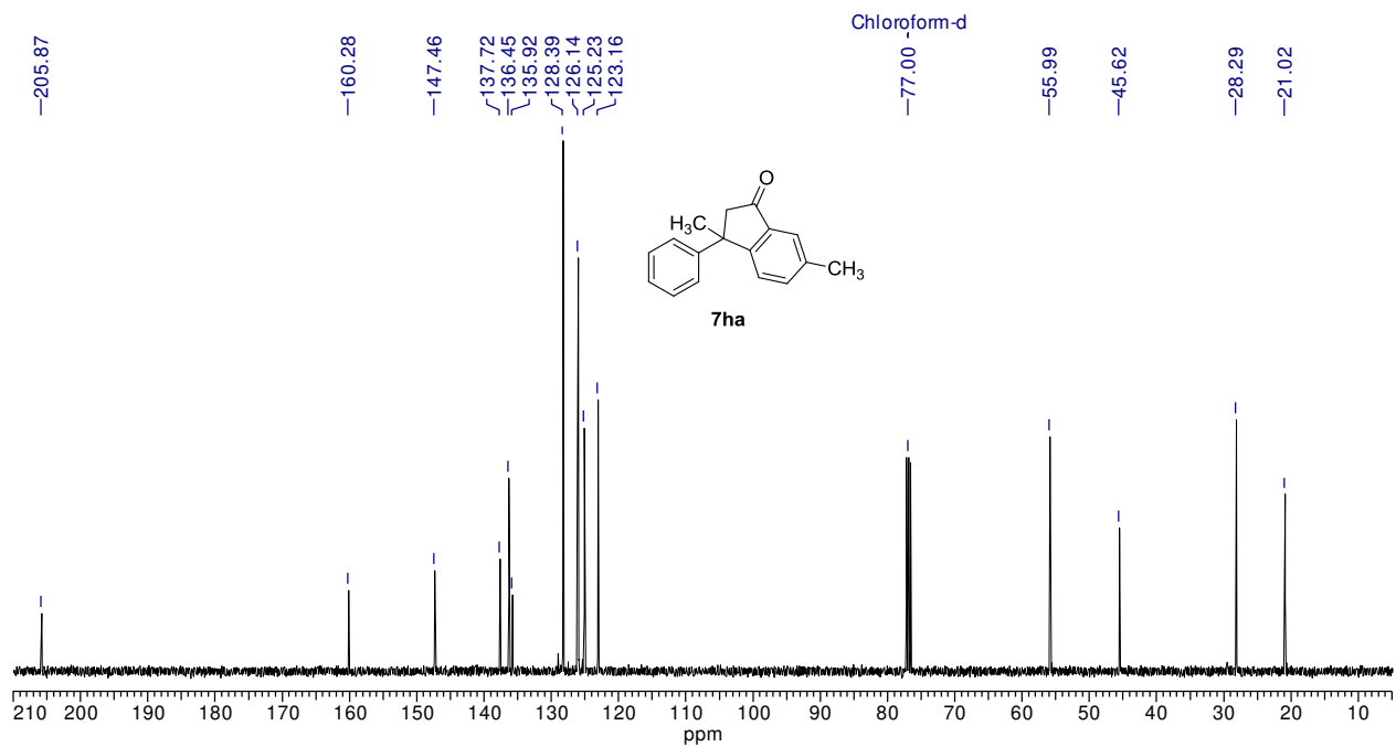
Figure I.12: 13 C-NMR (100 MHz) spectrum of 7ha in CDCl 3
