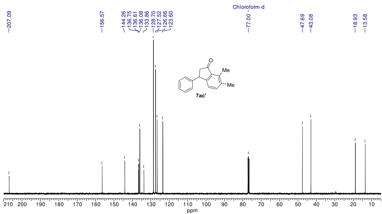
Figure I.17: ^{13}\text{C-NMR} (100 MHz) spectrum of 7ac' in \text{CDCl}_3
