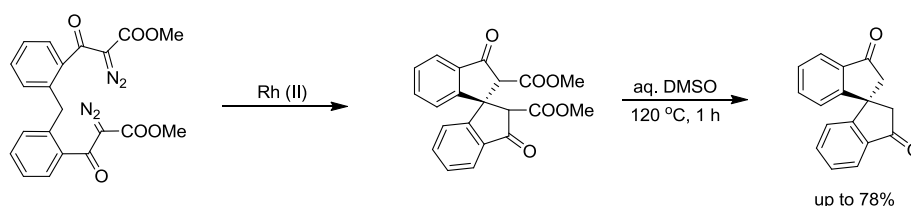
Scheme II.21
