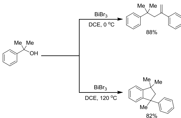
Scheme III.7
