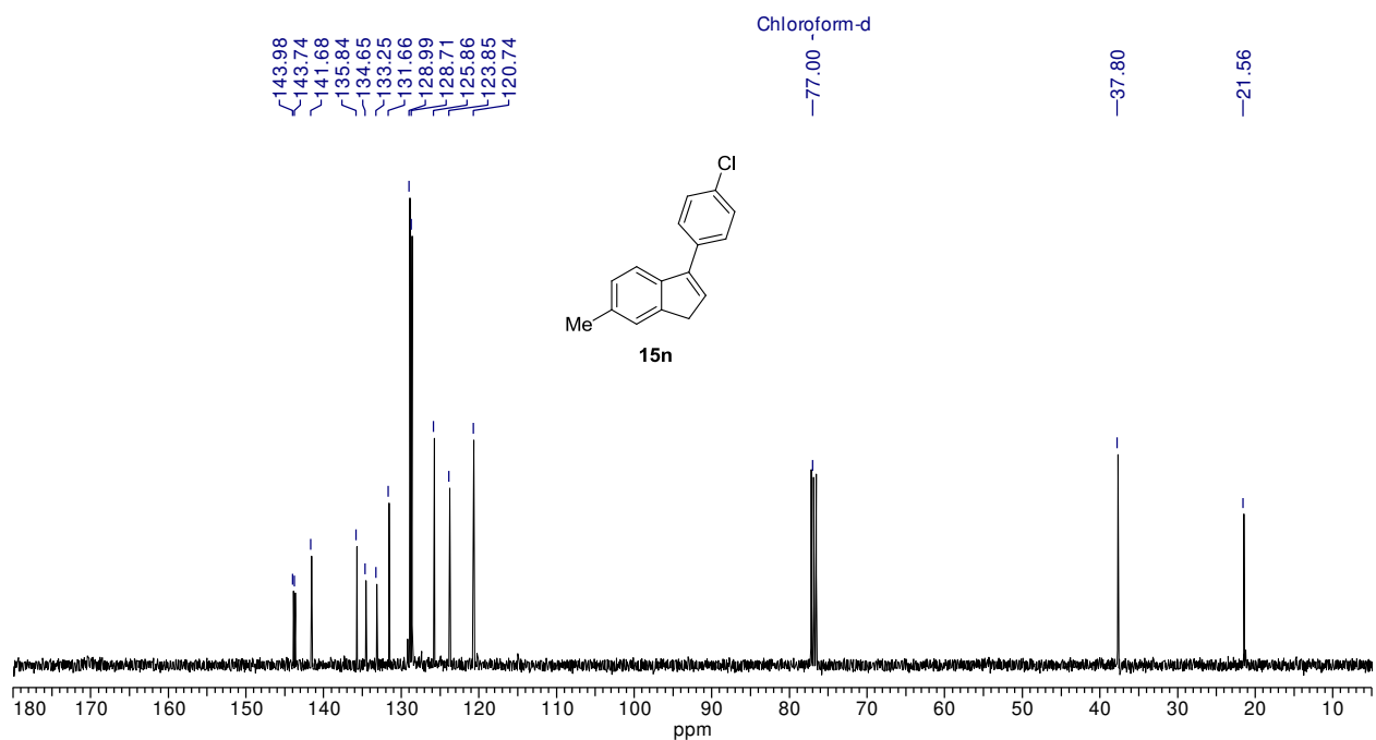
Figure II.18: 13 C-NMR (100 MHz) spectrum of 15n in CDCl 3
