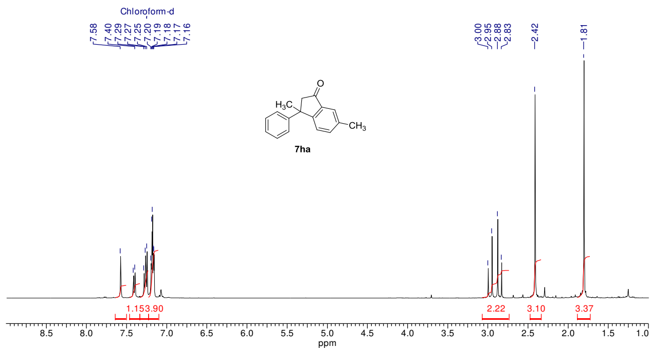
Figure I.11: 1 H-NMR (400 MHz) spectrum of 7ha in CDCl 3
