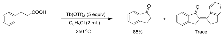
Scheme I.12
