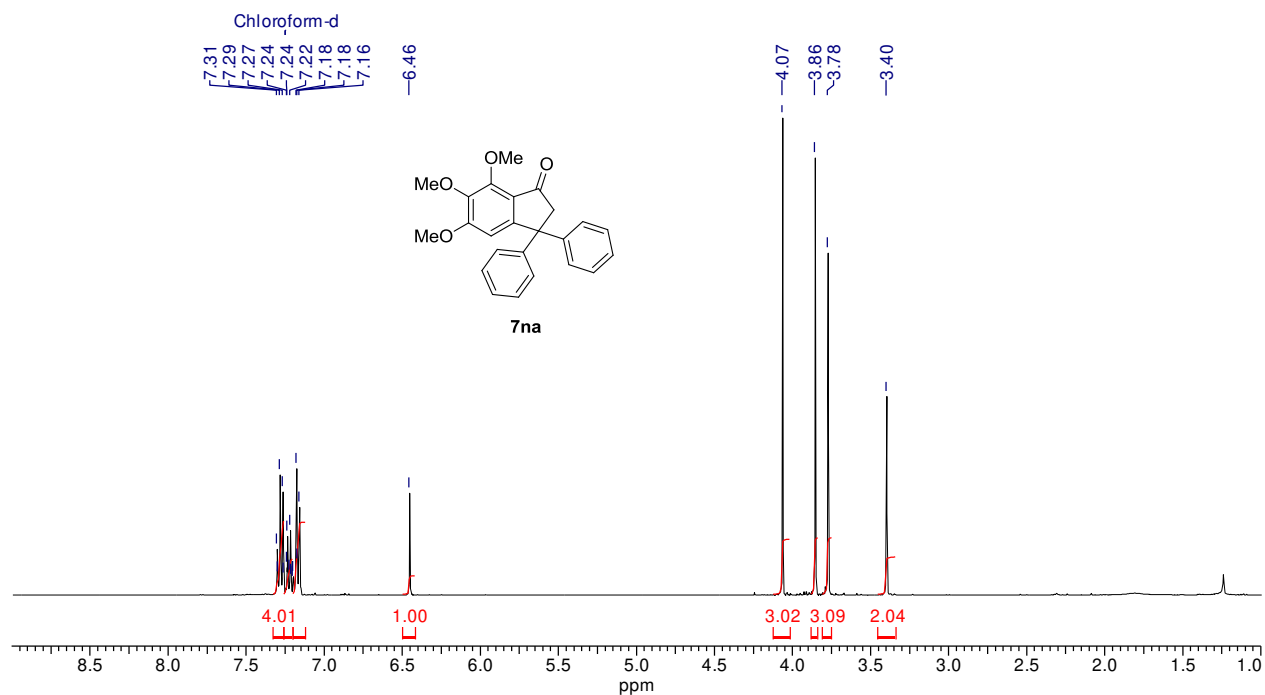
Figure I.14: ^1\text{H-NMR} (400 MHz) spectrum of 7na in \text{CDCl}_3
