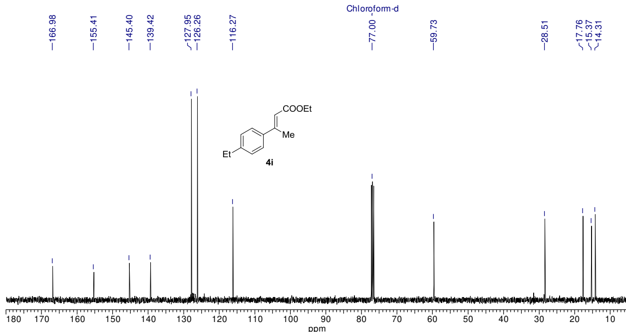
Figure I.8: ^{13}\text{C-NMR} (100 MHz) spectrum of 4i in \text{CDCl}_3
