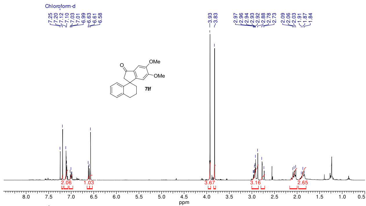
Figure I.18: ^1\text{H-NMR} (400 MHz) spectrum of 7lf in \text{CDCl}_3
