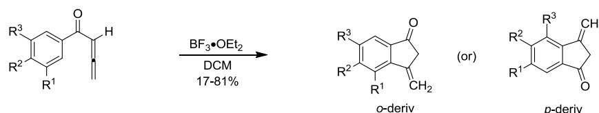
Scheme II.13
