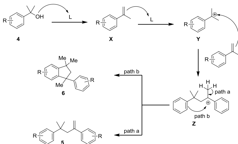
Scheme III.13
