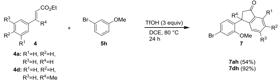
Scheme I.21
