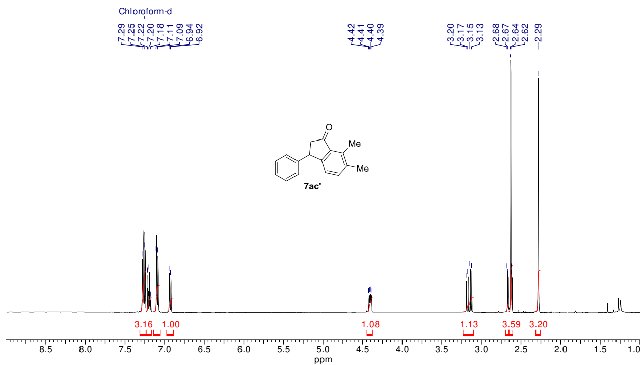
Figure I.16: ^1\text{H-NMR} (400 MHz) spectrum of 7ac' in \text{CDCl}_3
