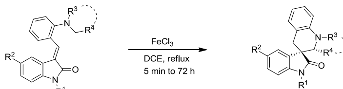
Scheme II.19
