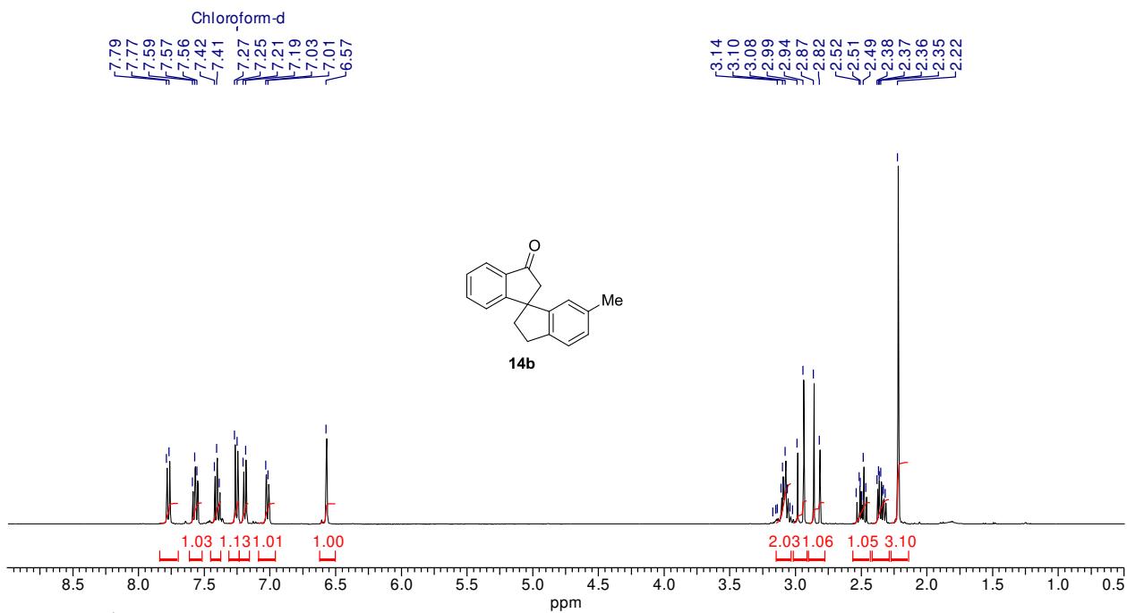
Figure II.27: ^1\text{H} -NMR (400 MHz) spectrum of 14b in \text{CDCl}_3
