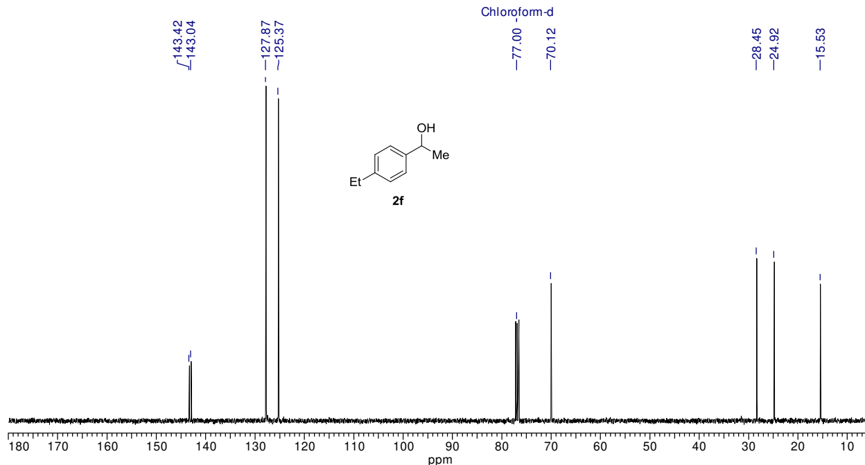
Figure I.4: 13 C-NMR (100 MHz) spectrum of 2f in CDCl 3
