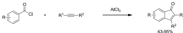
Scheme II.9
