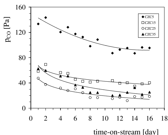
Figure 4: CO formation during SRM of four CZC catalysts as a function of time-on-stream ( m_{\text{CuO}} = 0.0225 g, T = 523 K, p = 10^5 Pa, w = 0.07 cm 3 min -1 , MeOH:H 2 O = 1:1)
