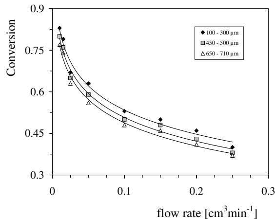
Figure 5: Methanol conversions during SRM as a function of the reactant flow rate, determined for various sieve fractions of CZC15 ( m = 0.5500 g, T = 523 K, p = 10^5 Pa, MeOH:H 2 O = 1:1)
