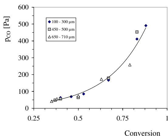
Figure 6: CO partial pressures determined for various sieve fractions of CZC15 during SRM under standard conditions ( m = 0.5500 g, T = 523 K, p = 10^5 Pa, MeOH:H 2 O = 1:1)
