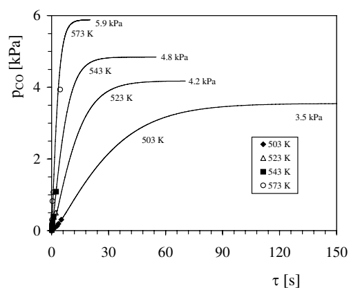
Figure 12: CO partial pressures during SRM of CZC15 as a function of contact time at different reaction temperatures ( m = 0.6726 g, p = 10^5 Pa, MeOH:H 2 O = 1:1)
