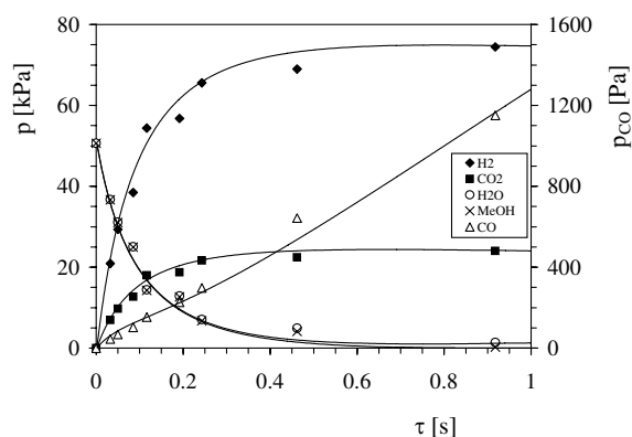
Figure 10: Partial pressures of the components in the reaction mixture during SRM on CZC15, experimental data and fitting results m = 0.6726 g, T = 573 K, p = 10^5 Pa, MeOH:H 2 O = 1:1
