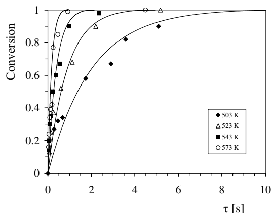
Figure 11: Methanol conversions during SRM of CZC15 as a function of contact time at different reaction temperatures ( m = 0.6726 g, p = 10^5 Pa, MeOH:H 2 O = 1:1)
