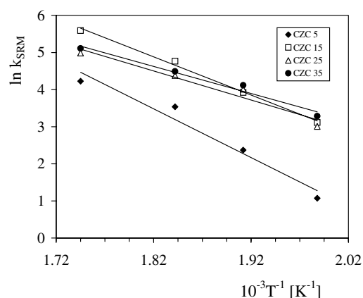
Figure 14: Arrhenius representation of the reaction rate constants obtained for the SRM reaction on the CZC catalysts
