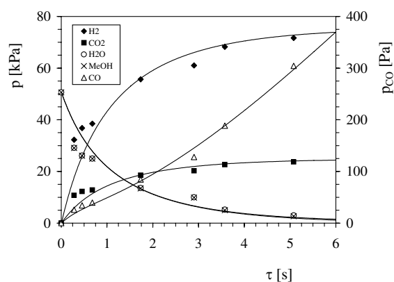
Figure 7: Partial pressures of the components in the reaction mixture during SRM on CZC15, experimental data and fitting results m = 0.6726 g, T = 503 K, p = 10^5 Pa, MeOH:H 2 O = 1:1
