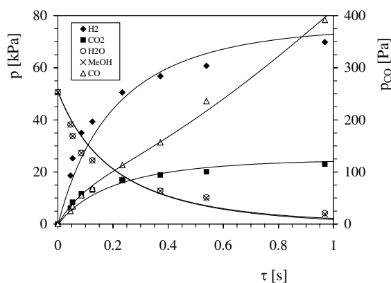
Figure 9: Partial pressures of the components in the reaction mixture during SRM on CZC15, experimental data and fitting results m = 0.6726 g, T = 543 K, p = 10^5 Pa, MeOH:H 2 O = 1:1
