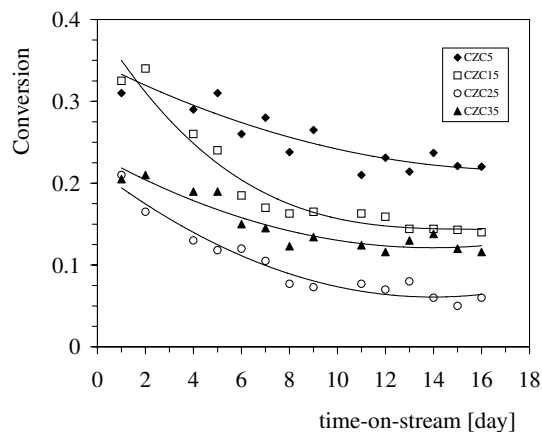
Figure 3: Methanol conversions during SRM of four CZC catalysts as a function of time-on-stream ( m_{\text{CuO}} = 0.0225 g, T = 523 K, p = 10^5 Pa, w = 0.07 cm 3 min -1 , MeOH:H 2 O = 1:1)
