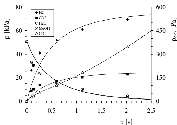
Figure 8: Partial pressures of the components in the reaction mixture during SRM on CZC15, experimental data and fitting results m = 0.6726 g, T = 523 K, p = 10^5 Pa, MeOH:H 2 O = 1:1
