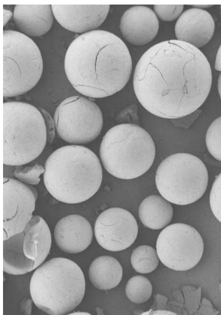
Figure 1: Scanning electron micrograph of a Cu/ZrO 2 /CeO 2 catalyst (CZC5) after calcination.
