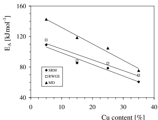
Figure 15: Apparent activation energies of the model reactions (SRM, RWGS, and MD) as a function of the Cu content of four CZC catalysts
