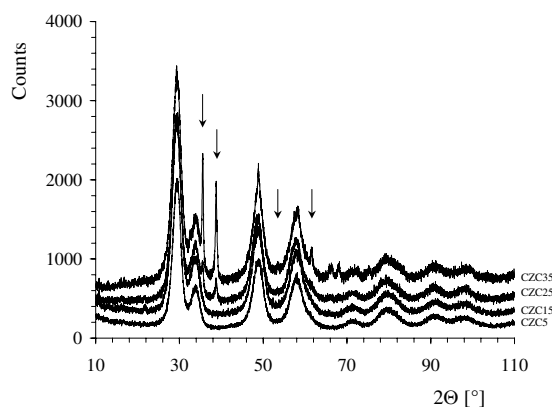
Figure 2: X-ray diffraction patterns of four CZC catalysts with a nominal copper concentration of 5% (CZC5), 15% (CZC15), 25% (CZC25), and 35% (CZC35) with a constant ZrO 2 /CeO 2 ratio of about 1. Arrows indicate CuO phase.
