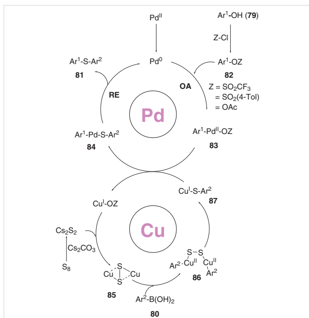
Scheme 20 Proposed mechanism for the synthesis of diaryl sulfides 81
