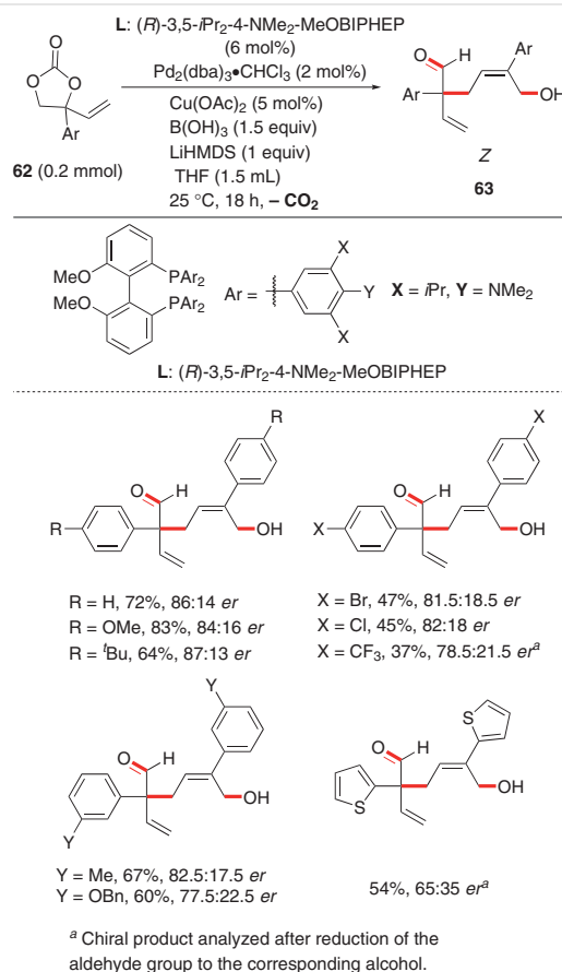
Scheme 14 Substrate scope for the synthesis of targets 63
