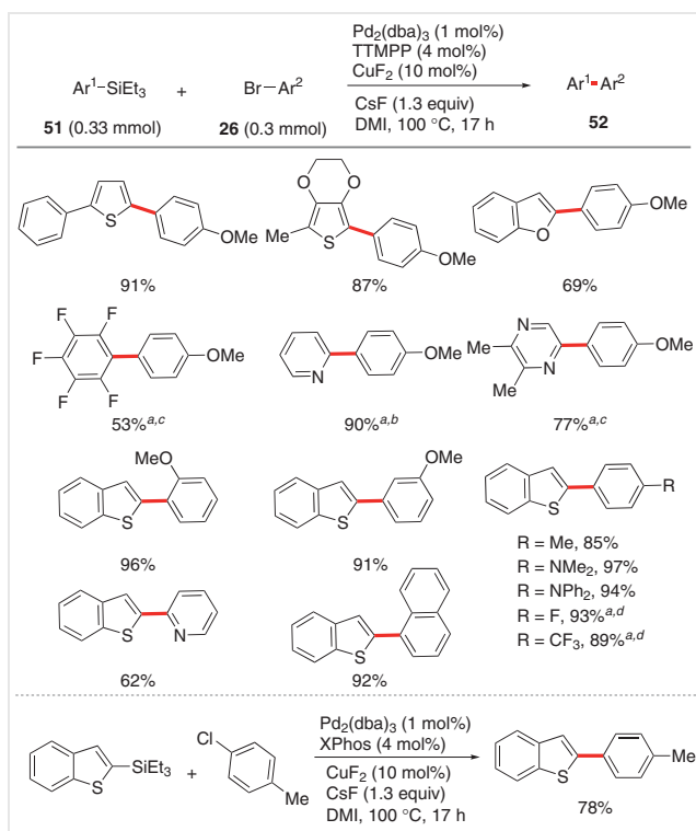
Scheme 12 Pd/Cu-catalysed cross-coupling of bromoarenes 26 and aryl(trialkyl)silanes 51 . a Reaction at 120 °C; b \text{PPh}_2(2\text{-NMe}_2\text{C}_6\text{H}_4) was used instead of TTMPP; c XPhos was used instead of TTMPP, heated at 120 °C; d JohnPhos was used instead of TTMPP.
