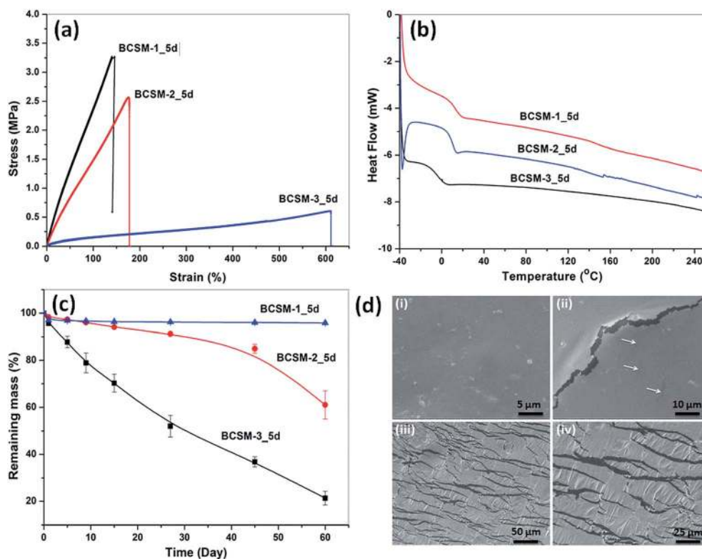
Fig. 3 Representative stress–strain plots of different polyesters with varying BHET contents after 5 days post-polymerization (a); DSC thermograms of different polyesters with varying BHET contents after 5 days post-polymerization (b); in vitro hydrolytic degradation profile of different polyesters with varying BHET contents after 5 days post-polymerization (c) and SEM images of degraded polyester film surfaces of BCSM-2 after 5 days post-polymerization (d) after 1 day (i), 7 day (ii) and 14 day; 300 \times mag. (iii) and 600 \times mag. (iv).
