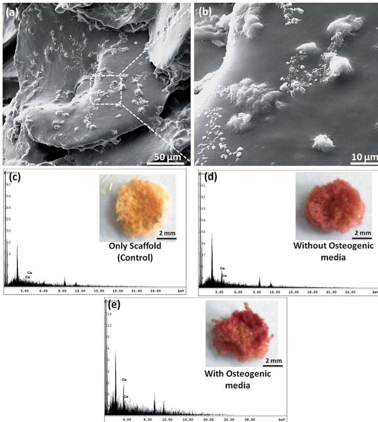
Fig. 7 SEM micrographs of 3D scaffold showing mineral deposition after 7 days of cell culture at 500 \times (a) and 2000 \times magnification (b). EDAX spectra of mineralized scaffold, before cell culture (c), cell culture without osteogenic supplement in media (d) and with osteogenic supplement in media (e) at 7 days with inset displaying the photograph of the scaffold stained with Alizarin Red S dye. The dimension of 3D scaffold was 6 mm diameter and 3 mm thickness.
