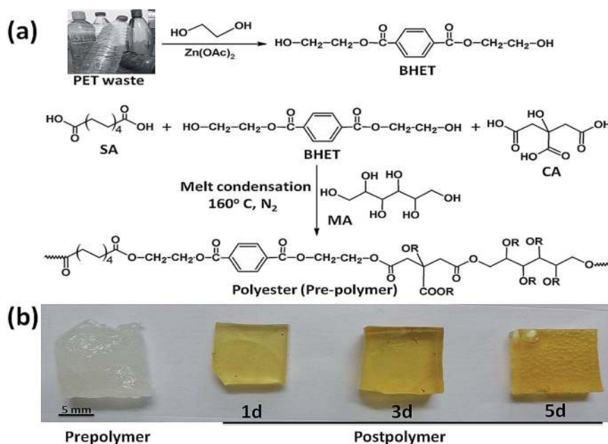
Fig. 1 (a) Synthesis scheme for preparation of BHET monomer and subsequently the pre-polymer, and (b) photographs of the polyester prior to post-polymerization (white, opaque) and after post-polymerization at different post-polymerization times, 1 day (light yellow, transparent), 3 days (brighter yellow, transparent) and 5 days (bright yellow, transparent).
