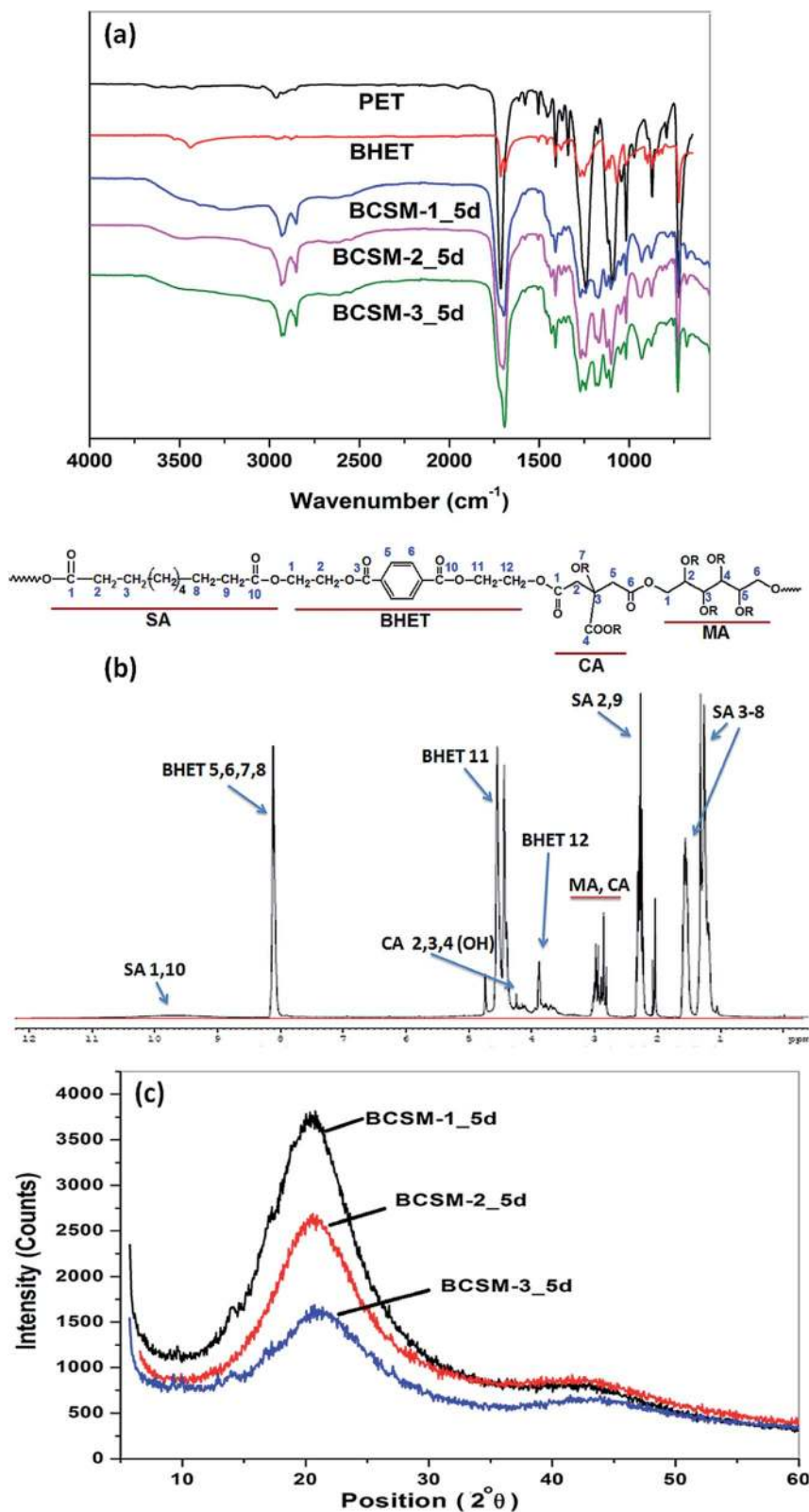
Fig. 2 Chemical characterization of different polyester elastomers at 5 days post-polymerization. FTIR spectra of PET, BHET and all polyesters at 5 days post-polymerization (a); ^1\text{H} NMR spectra of purified BCSM-2 pre-polymer (b) and X-ray diffraction patterns of all polyesters at 5 days post-polymerization (c).
