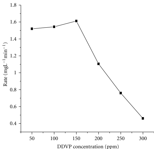
FIGURE 12: The effect of concentration of DDVP on the degradation of dichlorvos by \text{Mg}^{2+} -doped \text{TiO}_2 , pH = 2, catalyst dosage = 0.10 g.
