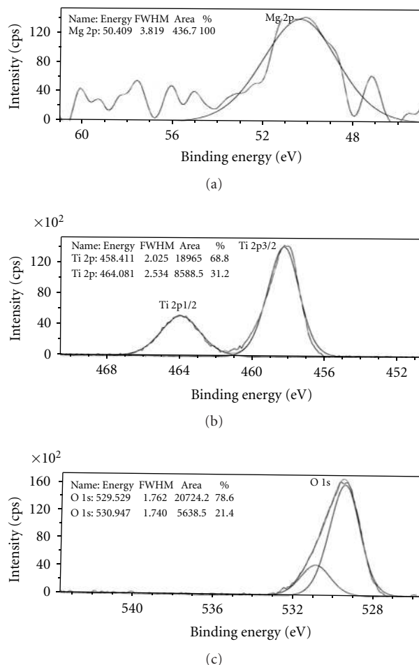
FIGURE 6: (a) High resolution of Mg 2p spectrum, (b) high resolution of Ti 2p spectrum, and (c) high resolution of O 1s spectrum.
