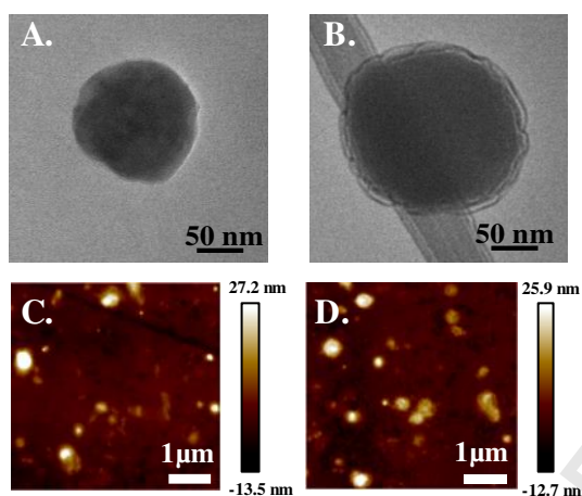
Fig. 3: Transmission electron microscopy (TEM) imaging of, A. NioIR; B. NioIR-C.; Atomic force microscopy imaging (AFM) of, C. NioIR; D. NioIR-C.
