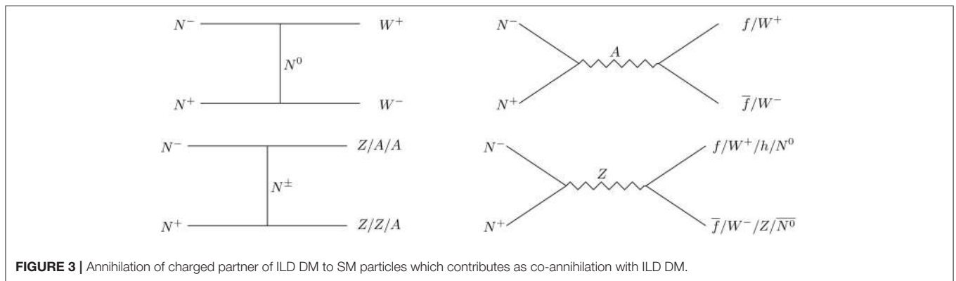
FIGURE 2 | Annihilation of ILD DM to SM particles.
