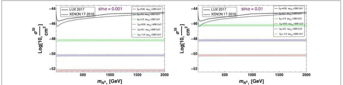
FIGURE 13 | SI direct detection cross-section \sigma^{SI} as a function of DM mass m_{N^0} for \sin \alpha = 0.001 (Left) and \sin \alpha = 0.01 (Right). Different choices of the coupling \{f_N = 0.01, 0.1, 1\} are shown in Red, Blue, and Green color, respectively. Dashed and solid lines corresponds to different values of the heavy Higgs m_{H_2} = 600, 280 GeVs, respectively. The bound from LUX 2017 and XENON1T 2018 are shown.
