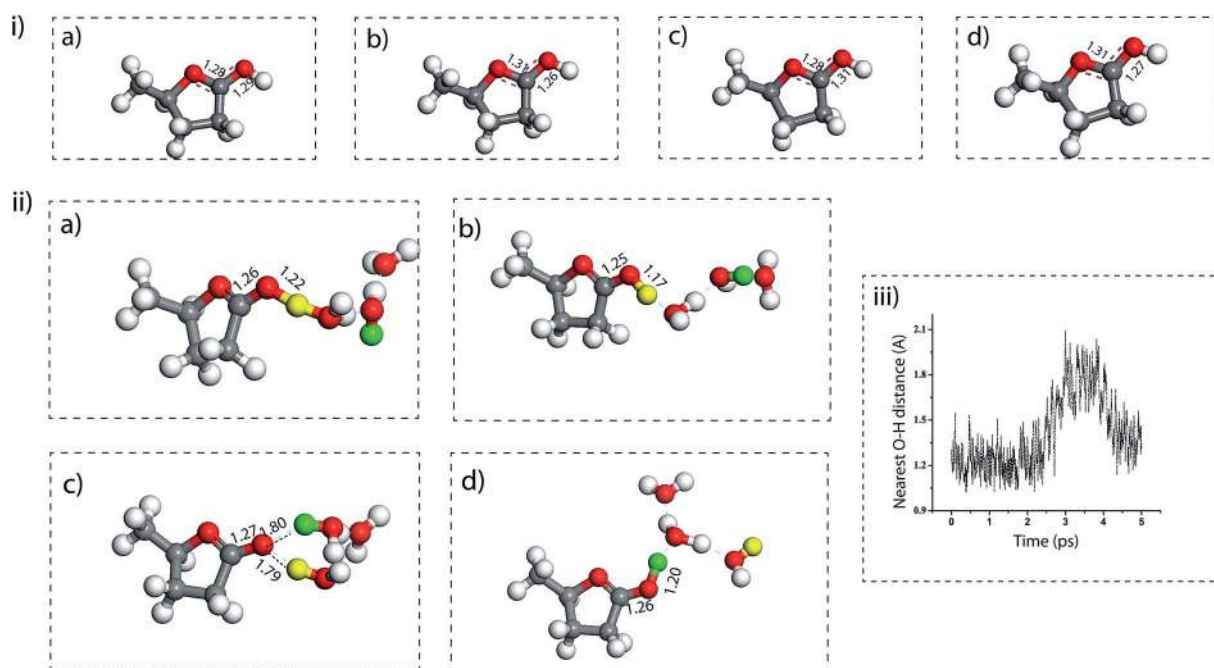
Fig. 6 AIMD simulation of the oxocarbenium ion of GVL in (i) implicit and (ii) explicit water environment. (iii) Nearest hydrogen distance from carbonyl oxygen of GVL during ab initio MD simulation in explicit water.
