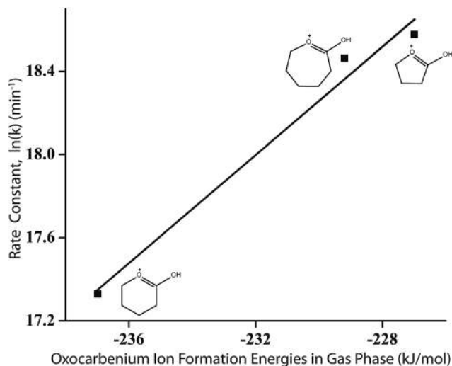
Fig. 5 Reaction rate constant for ring-opening of lactone molecules versus the respective gas-phase oxocarbenium ion formation energies.
