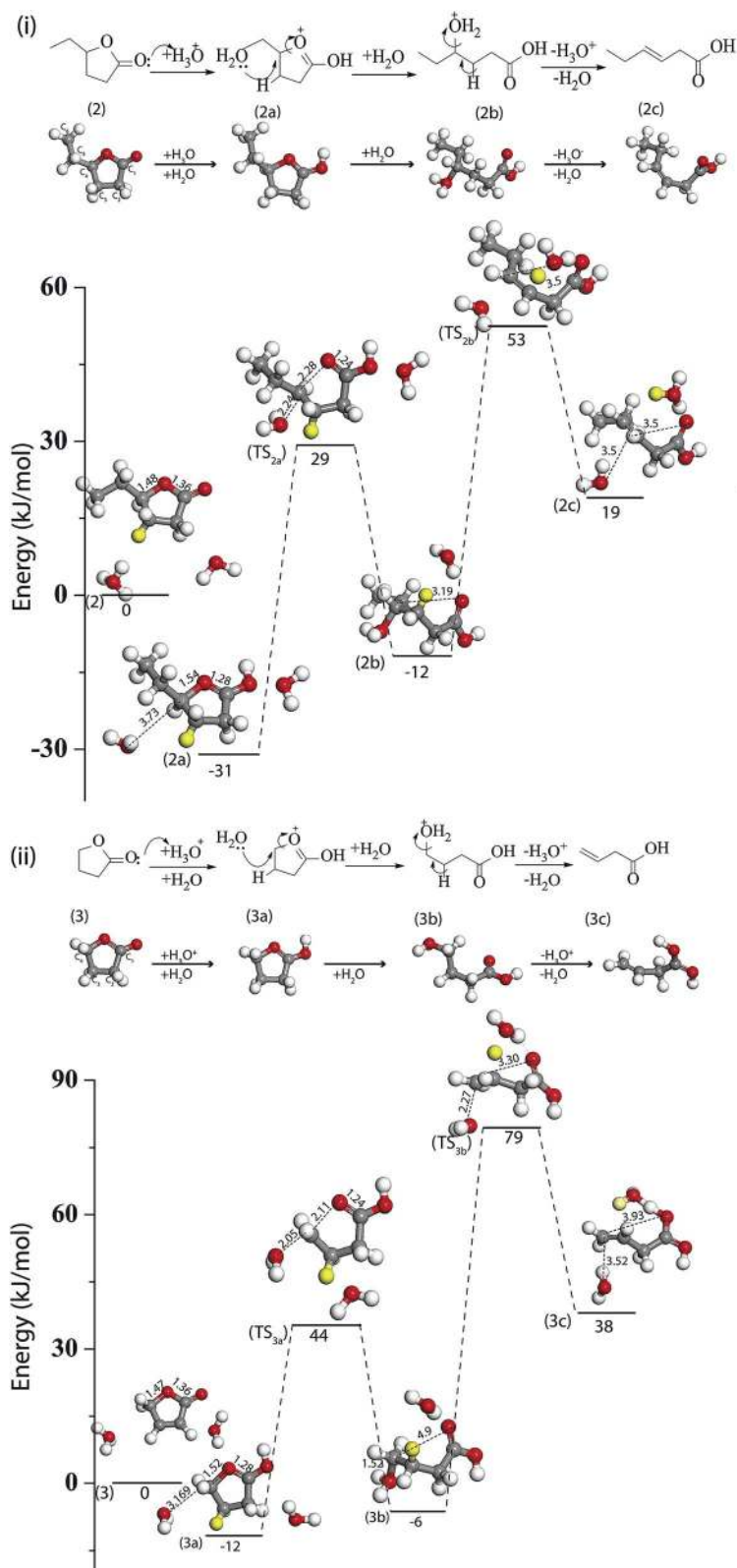
Fig. 3 DFT calculated energy diagram for the ring-opening of (i) GCL to form hex-3-en-oic acid and (ii) GBL to form but-3-en-oic acid.
