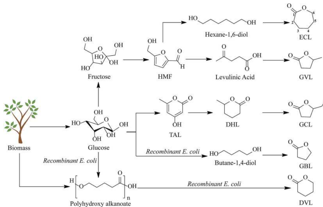
Fig. 1 Routes for the synthesis of biomass derived lactone molecules included in this study: \epsilon -caprolactone (ECL), \gamma -valerolactone (GVL), \gamma -caprolactone GCL, \gamma -butyrolactone (GBL) and \delta -valerolactone (DVL).
