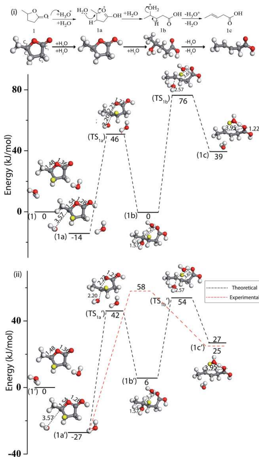
Fig. 2 DFT calculated energy diagram for GVL ring-opening to pentenoic acid.
