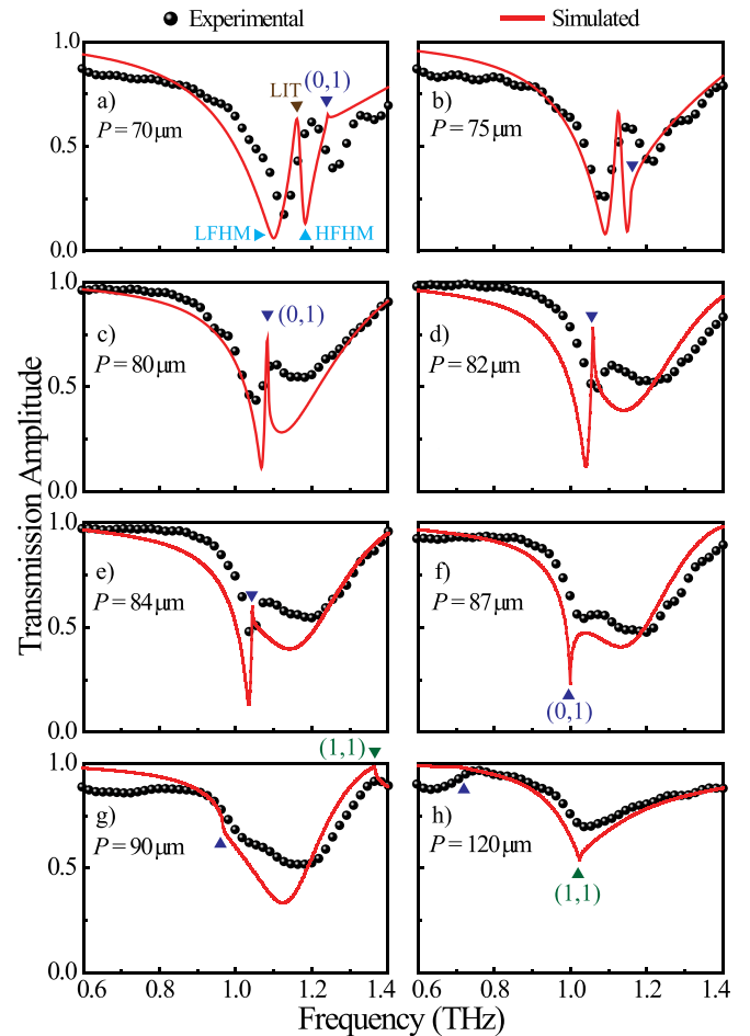
FIG. 2. (a)–(h) Experimental (black spheres) and simulated (red solid lines) transmission amplitude of the TASR metamaterial array with varying lattice period P = 70, 75, 80, 82, 84, 87, 90, and 120 \mu\text{m} , respectively. The low frequency hybrid mode (LFHM), high frequency hybrid mode (HFHM) and lattice induced transparency (LIT) are indicated in (a). The fundamental lattice mode (0,1) is marked by a dark blue triangle and the (1,1) order lattice mode is indicated by a green triangle.
