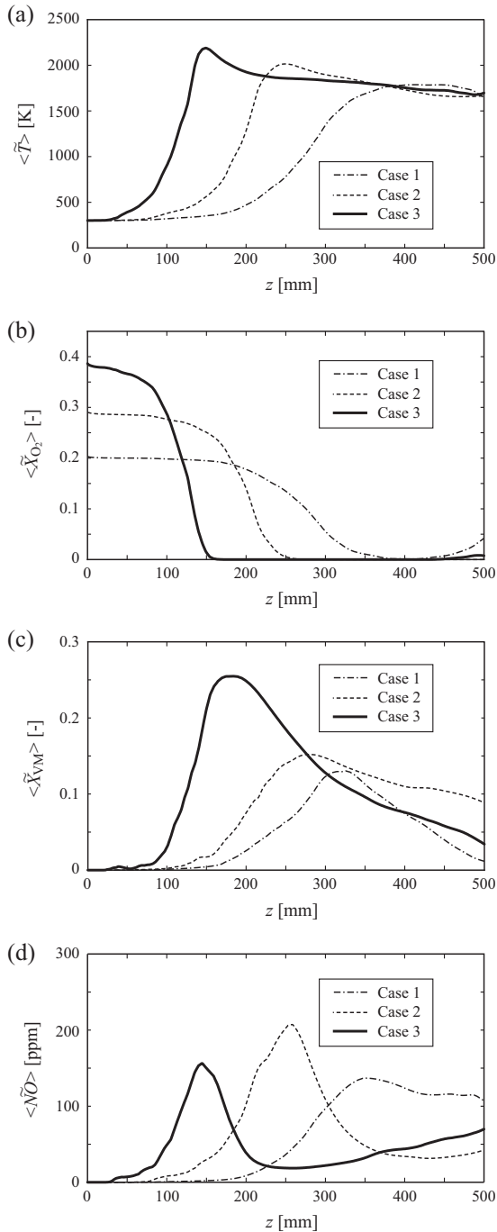
Fig. 9. Time-averaged axial distributions of (a) gas temperature \langle \bar{T} \rangle , and mole fractions of (b) O_2 ( \langle \bar{X}_{O_2} \rangle ), (c) volatile matter ( \langle \bar{X}_{VM} \rangle ) and (d) NO concentration ( \langle \bar{NO} \rangle ) at equivalence ratio of 1.73.
