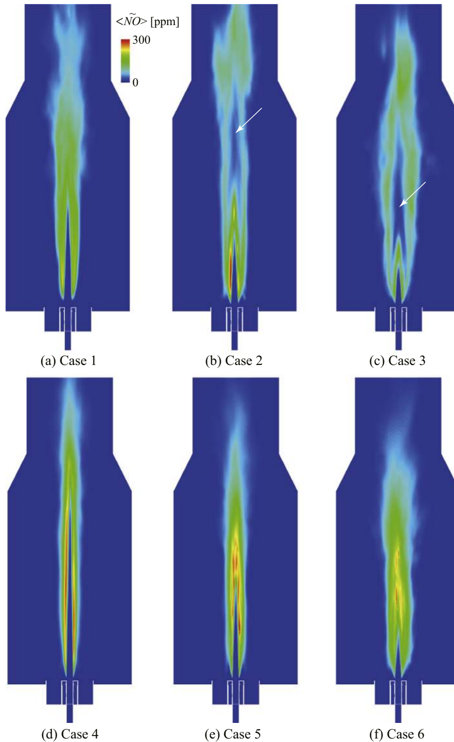
Fig. 7. Time-averaged distributions of NO concentration ( \overline{NO} ) on the x - z plane at y = 0 mm.
