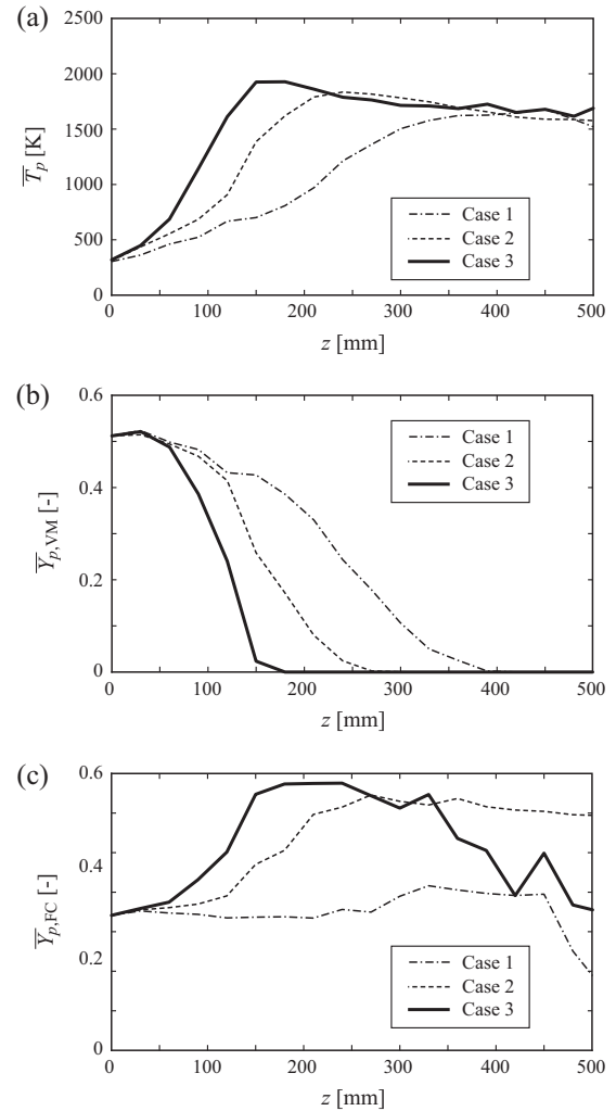
Fig. 10. Time-averaged axial distributions of (a) particle temperature \bar{T}_p , and mass fractions of (b) volatile matter \bar{Y}_{p,VM} and (c) fixed carbon \bar{Y}_{p,FC} in coal particles at equivalence ratio of 1.73.
