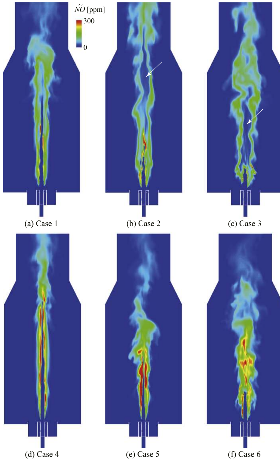
Fig. 6. Instantaneous distributions of NO concentration \bar{N}\bar{O} on the x - z plane at y = 0 mm.
