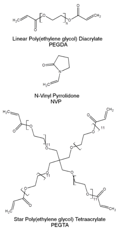
Figure 1. Chemical structure of poly(ethylene glycol) diacrylate (PEGDA) and the secondary reactive species (SRS) used in this study namely, namely N-vinyl pyrrolidone (NVP) and star poly(ethylene glycol) tetraacrylate (PEGTA).
