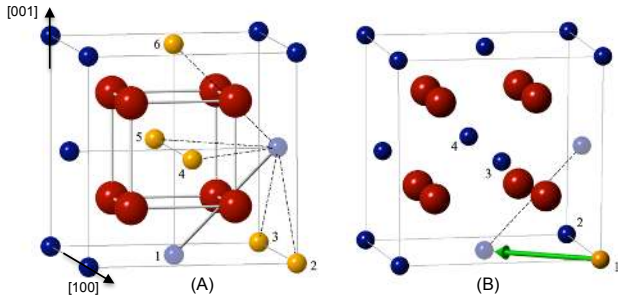
FIG. 6. (A) The six distinct di-vacancy configurations within first nearest neighbors in UO_2 unit cell, all other possibilities would be a simple translation of the above six configurations. (B) The four possible sites a single di-vacancy can hop to in order to maintain a di-vacancy pair.
