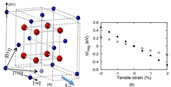
FIG. 9. (A) Schematic showing the applied strain along the [100] direction with the black arrow points towards the uranium vacancy possible migrations along the [110] and [011] directions. (B) Change in the migration barrier \Delta E_{\text{mig}} for V_U^x under applied uniaxial tensile strain along [100] for migration path oriented along [110] (open diamonds) and [011] directions (solid diamonds).
