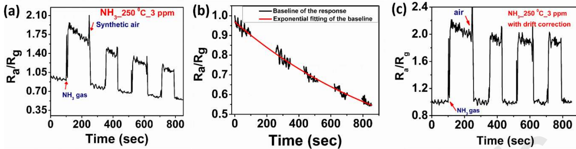
Figure 3. (a) Repeatability of the sensor for exposure of 4 cycles of 3 ppm ammonia at 250 °C; (b) Exponential fitting of the baseline; (c) Response after baseline correction.
