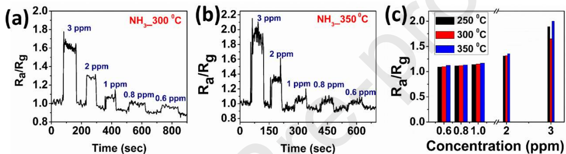
Figure 4. Dynamic response of sensor at (a) 300 °C and (b) 350 °C; (c) Comparison of response at various temperatures.
