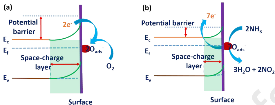
Figure 5. The principle of gas sensing with ZnO nanoflakes in (a) ambient air and (b) \text{NH}_3
