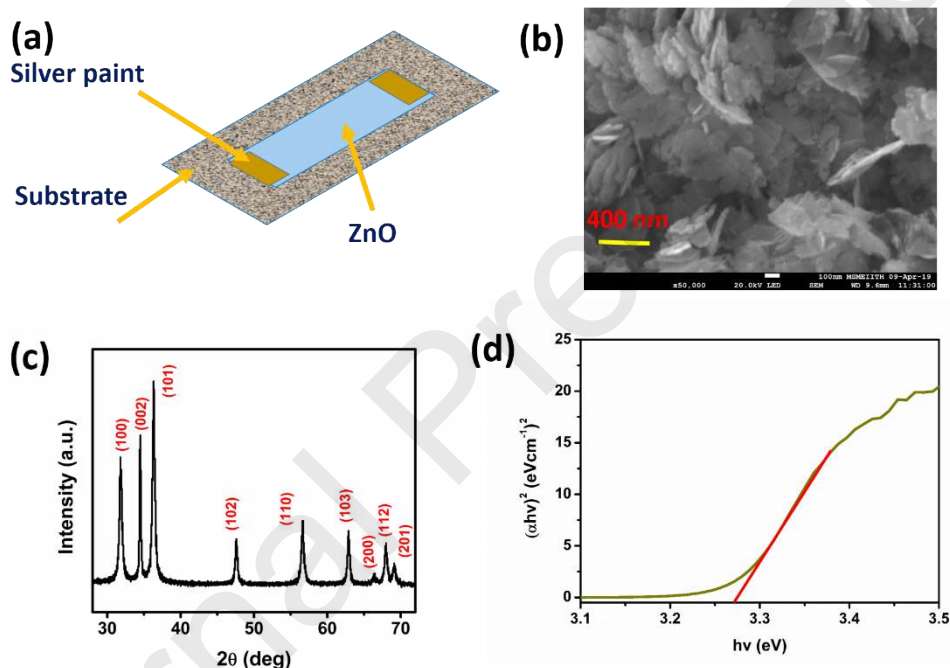
Figure 1. (a) ammonia sensor schematic; (b) Micrograph; (c) XRD; and (d) Tauc plot of 2D ZnO NFs
