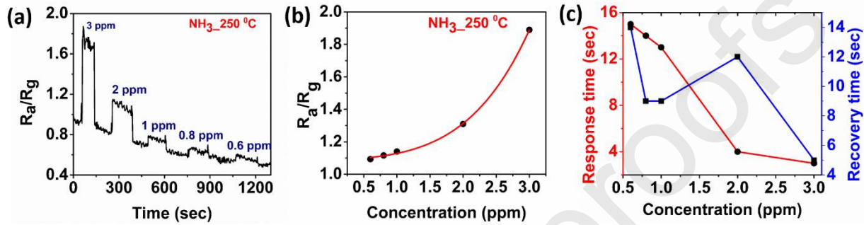
Figure 2. (a) Response of the sensor with NH_3 at 250\text{ }^\circ\text{C} ; (b) Response of the sensor with respect to gas concentration; (c) Response/recovery times of the sensor with different concentrations
