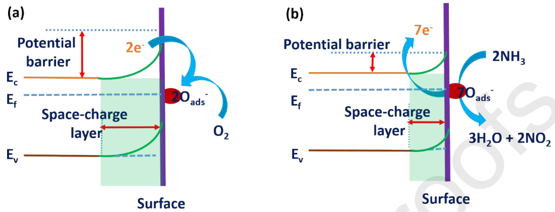
Ammonia gas sensing with 2D ZnO nanoflakes based chemiresistive sensor
