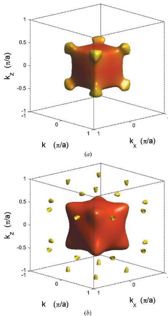
Figure 10 The calculated QSGW Fermi surface of ThTe in the B2 structure, with spin-orbit coupling included. In (a) the centre of the cubic Brillouin zone corresponds to the R -point ( \pi/a(1, 1, 1) ), i.e. the first sheet corresponds to hole pockets around the R -point. In (b) the centre corresponds to the \Gamma point, and the second sheet corresponds to a large electron pockets around \Gamma with some additional small pockets at the Brillouin zone faces. The colouring is only for presentation purposes.
