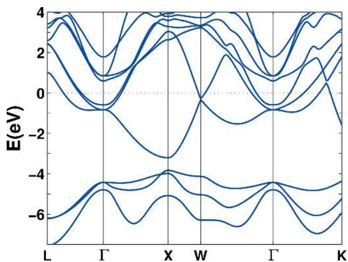
Figure 7 Band structure of ThSb in the ambient B1 crystal structure, as calculated in the QSGW approximation and with spin-orbit coupling included. The zero of energy is placed at the Fermi level.
