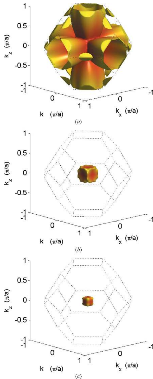
Figure 6 The calculated QSGW Fermi surface of ThSb, with spin-orbit coupling included. The first sheet (a) may be viewed as large electron ellipsoids centred at the X -points and merging together at the \Gamma -point. The second (b) and third (c) sheets are electron pockets around \Gamma . The first Brillouin zone is indicated by thin dotted lines. The colouring is only for presentation purposes.
