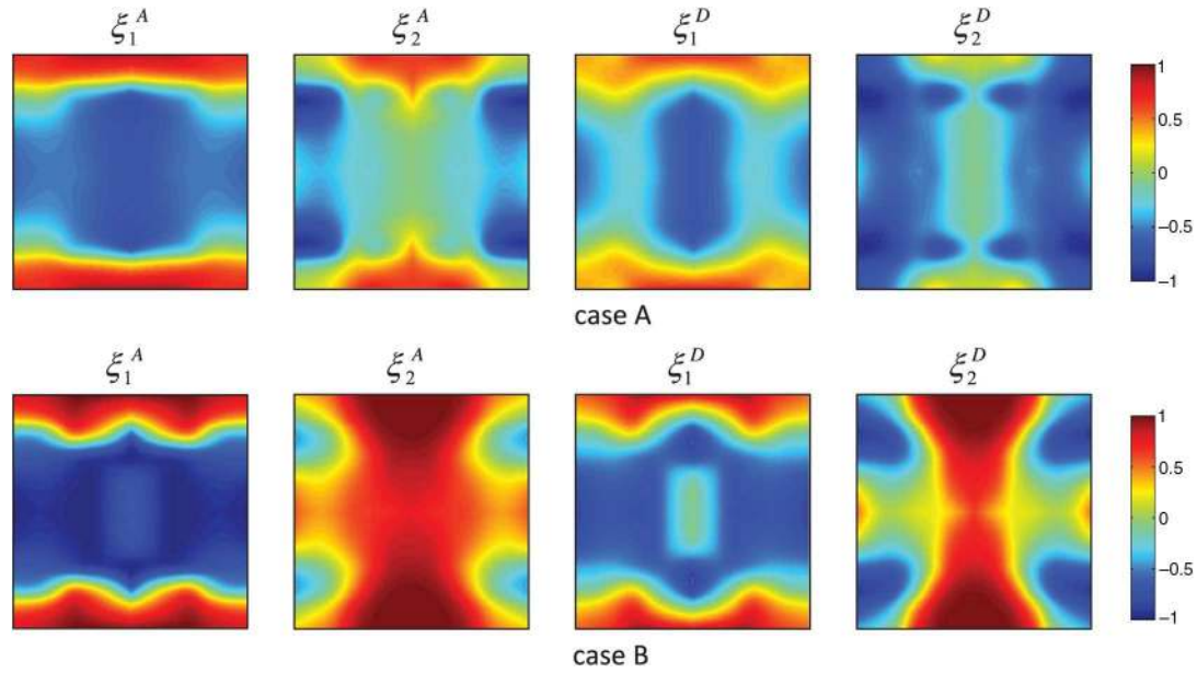
Fig. 6 Optimal lamination parameter distribution for a square VAT plate under two different in-plane boundary conditions (case A and case B): 7 \times 7 control points.
