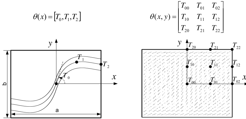
Fig. 3 Two illustrations for the nonlinear variation of fiber-orientation angles over the VAT plate domain. The fiber angles are parabolically varying along either x direction (left) or both axes directions (right).
