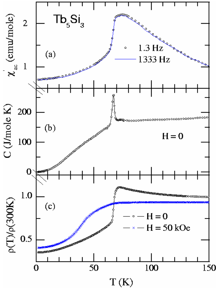
Figure 1: (color online) (a) Real part of ac \chi , (b) heat-capacity ( C ), and (c) normalized electrical resistivity ( \rho ) as a function of temperature for Tb_5Si_3 . We have also plotted the \rho data in the presence of 50 kOe. In the case of C(T) figure, a line is drawn through the data points.
