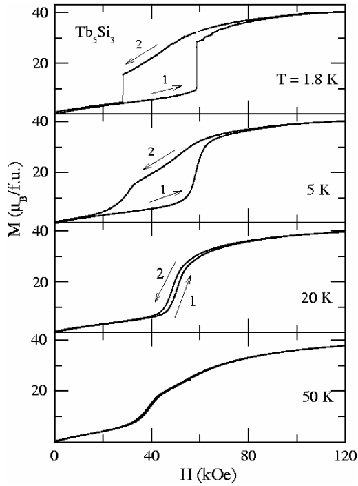
Figure 2: Isothermal magnetization behavior at several temperatures for Tb_5Si_3 . The numerals near the curves serve as guides to the eyes.
