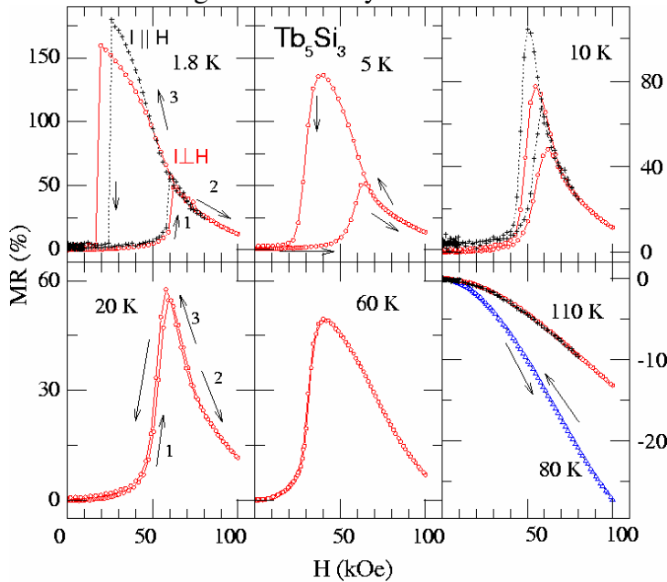
Figure 3: (color online) Magneto-resistance, defined as [\rho(H)-\rho(0)]/\rho(0) , as a function of magnetic field for Tb_5Si_3 for transverse geometry of current and field directions (data points with continuous lines through them). For some temperatures, the curves (dotted lines through points marked '+') are shown for longitudinal geometry. The arrows and numbers placed near these (shown in some graphs only) serve as guides to the eyes.
