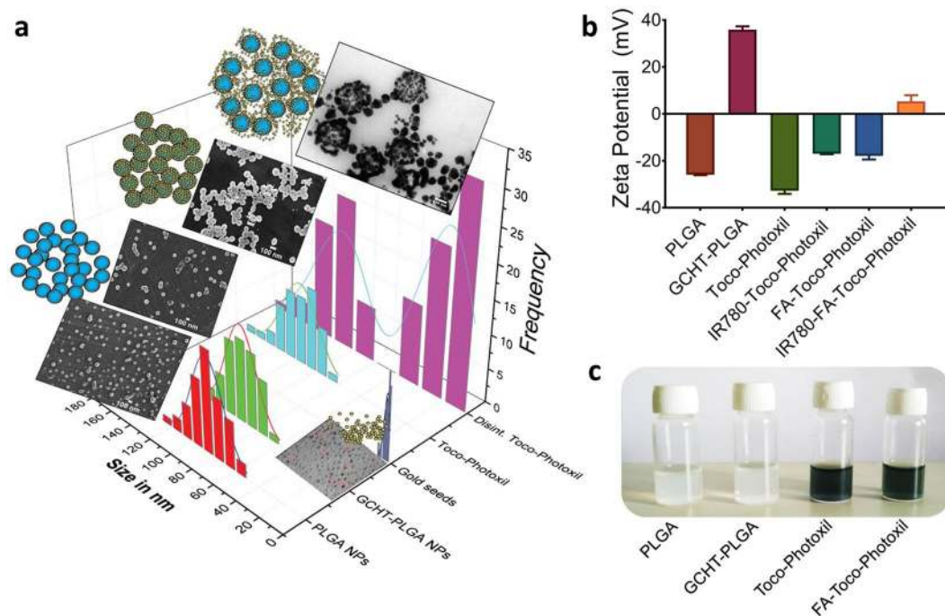
Figure 2. Characterization of nanoformulations. (a) Size distribution of nanomaterials synthesized at different stages overlapped with their representative FEG-SEM and FEG-TEM images. (b) Graph shows the zeta potential values of the various nanoformulations. (c) Representative photograph of PLGA NPs, GCHT-PLGA NPs, Toco-Photoxil, and FA-Toco-Photoxil nanoformulations.
