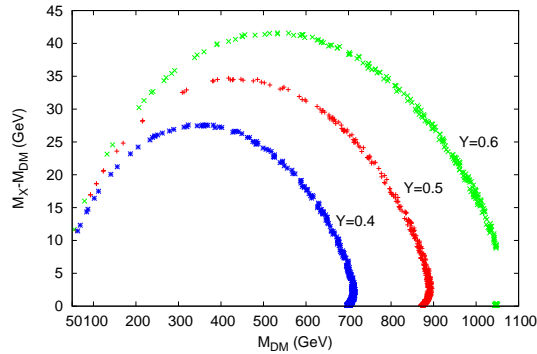
FIG. 6: Observed relic abundance in the plane of M_X - M_{DM} versus M_{DM} for different values of the couplings, i.e., Y = 0.4, 0.5, 0.6 .
