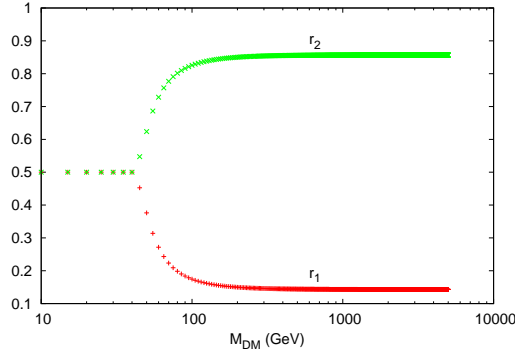
FIG. 4: r_1 and r_2 as a function of M_{\text{DM}} for Y_{\Sigma} = Y_H . For simplicity we set M_{\text{DM}} = M_X .
