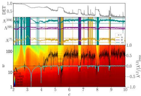
Fig. 6 DET, single scale-specific lacunarities \Lambda^{(w)} and RL curves for varying c \in [2, 10] with n = 2000 for the Roessler system. 95% – confidence bounds are obtained via bootstrapping and excursions outside the indicated horizontals are indicated. Each time series has T = 1000 values after discarding transients. In the lower panel, w –axis and color coding are scaled logarithmically. Black (cyan) curves display the first (second) Lyapunov exponent normalized to their maximum absolute values for better visibility
