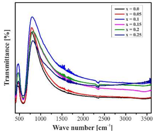
Fig. 4. FT-IR spectra of \text{Co}_{1-x}\text{Mg}_x\text{Fe}_2\text{O}_4 powder samples annealed at 1100\text{ }^\circ\text{C} for 2 h.
