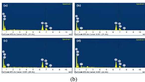
Fig. 3. (a) Scanning electron micrographs of \text{Co}_{1-x}\text{Mg}_x\text{Fe}_2\text{O}_4 powder samples annealed at 1100\text{ }^\circ\text{C} for 2 h; (b) EDX patterns of \text{Co}_{1-x}\text{Mg}_x\text{Fe}_2\text{O}_4 powder samples annealed at 1100\text{ }^\circ\text{C} for 2 h.
