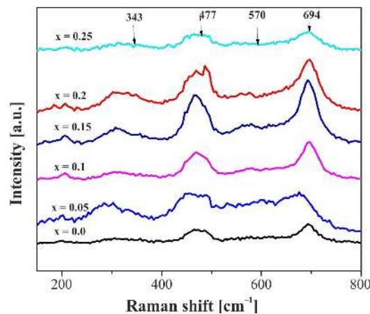
Fig. 5. Raman spectra of \text{Co}_{1-x}\text{Mg}_x\text{Fe}_2\text{O}_4 powder samples annealed at 1100\text{ }^\circ\text{C} for 2 h.
