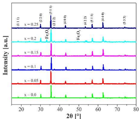
Fig. 1. X-ray diffraction patterns of \text{Co}_{1-x}\text{Mg}_x\text{Fe}_2\text{O}_4 powder samples annealed at 1100 \text{ }^\circ\text{C} for 2 h.
