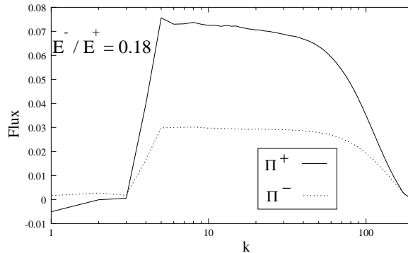
FIG. 1. Energy fluxes \Pi^\pm versus k for a two-dimensional run with B_0 = 0.0 and E^-/E^+ = 0.18 . Here \Pi^+ > \Pi^- . The figure is taken from Dar [3].
