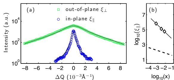
FIG. 1: (Color online) (a) Line profiles through the CDW satellite peak in 1T -TaS 2 in the out-of-plane and in-plane directions. Solid lines are best fits to Lorentzian line shapes. (b) \xi_{\parallel} versus doping ( x ) compared with strong- (dashed line) and weak-pinning (solid line) functional forms.
