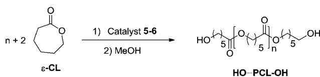
Scheme 6 Ring-opening polymerisation of \epsilon -CL with strontium and barium complexes 5 and 6 .
