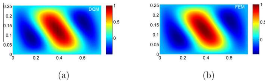
Fig. 9. Rectangular VAT plate [60_2, 60 \pm (90|10)]_s subjected to in-plane negative shear load: Buckling mode shape (a) DQM (b) FEM.
