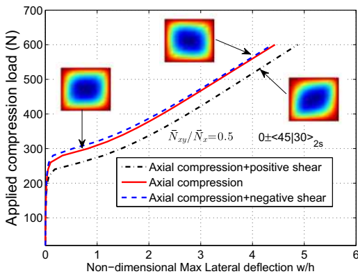
Fig. 25. Square VAT plate 0 \pm (45|30)_{2s} subjected to combined axial compression and shear load with load ratio \bar{N}_{xy}/\bar{N}_x = 0.5 .
