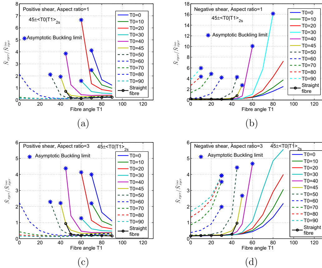
Fig. 14. Square VAT plate 45 \pm (T_0/T_1)_{2s} subjected to in-plane shear displacement (a) positive shear, aspect ratio = 1 (b) negative shear, aspect ratio = 1 (c) positive shear, aspect ratio = 3 (d) negative shear, aspect ratio = 3.
