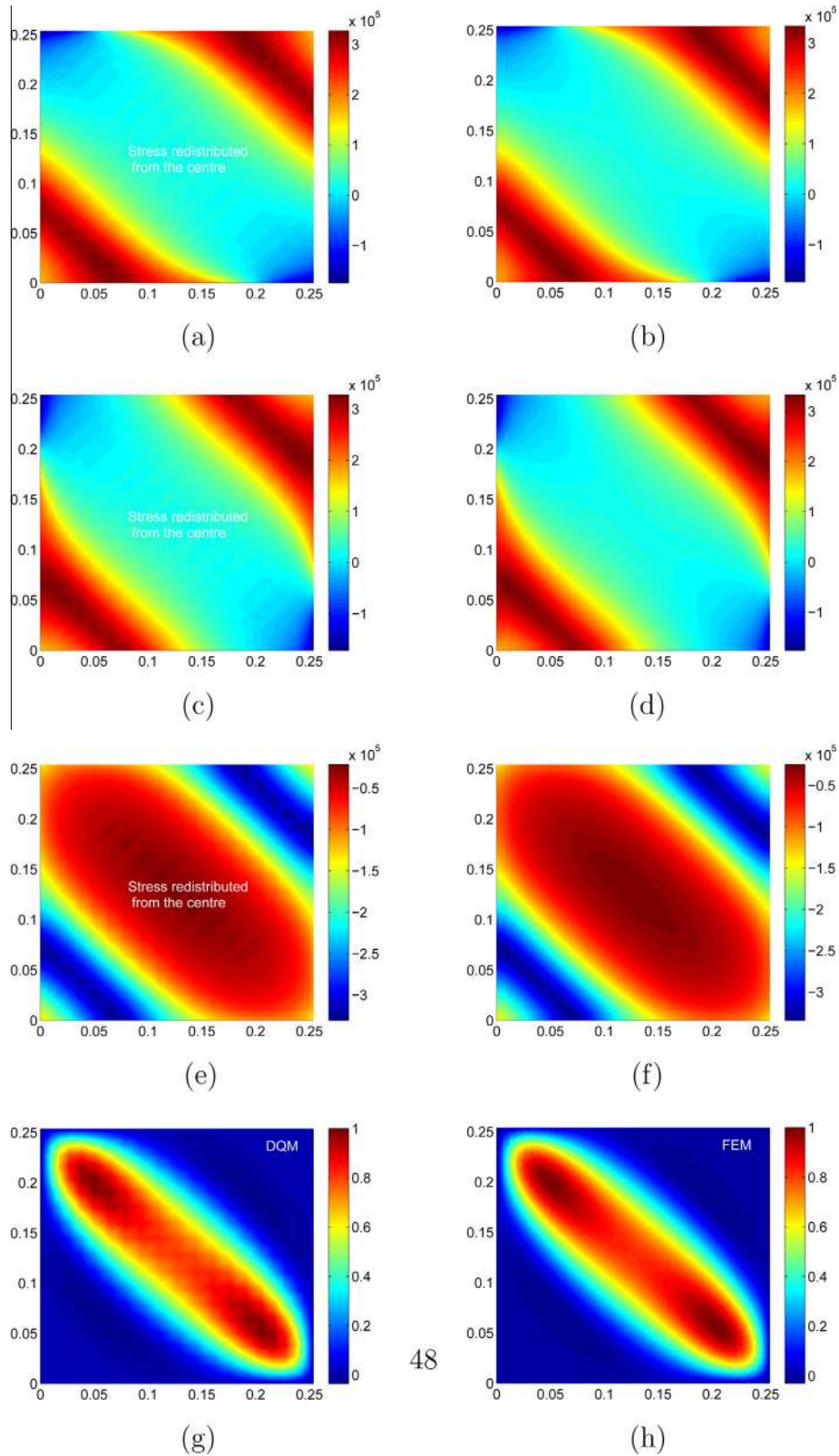
Fig. 15. Square VAT plate [45 \pm (30/80)]_2 , subjected to in-plane negative shear displacement: stress resultant distribution \bar{N}_x (a) DQM (b) FEM, stress resultant distribution \bar{N}_y (c) DQM (d) FEM, stress resultant distribution \bar{N}_x (e) DQM (f) FEM, buckling mode shape (g) DQM (h) FEM.
