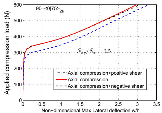
Fig. 26. Square VAT plate 90 \pm (0|75)_{2s} subjected to combined axial compression and shear load with load ratio \bar{N}_{xy}/\bar{N}_x = 0.5 .
