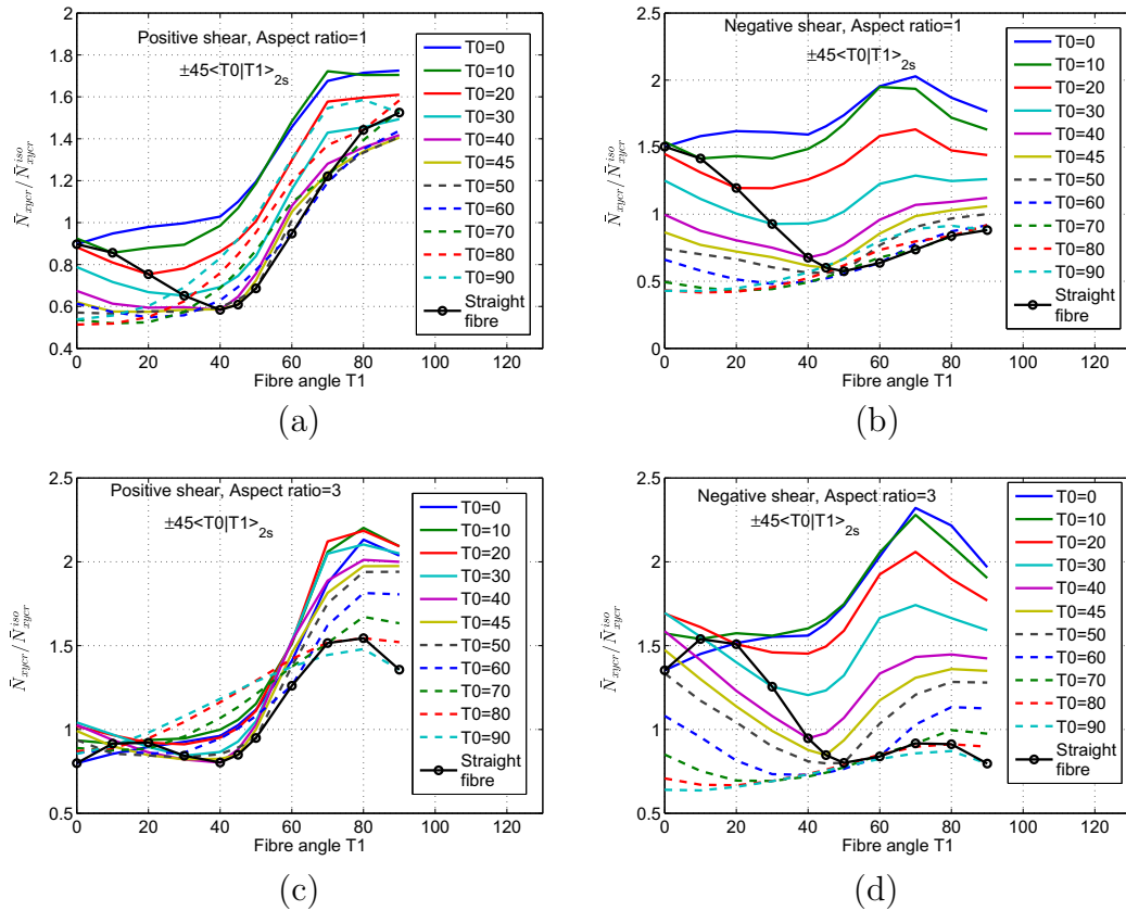
Fig. 13. Square VAT plate \pm 45\langle T_0 | T_1 \rangle_{2s} subjected to in-plane shear displacement (a) positive shear, aspect ratio = 1 (b) negative shear, aspect ratio = 1 (c) positive shear, aspect ratio = 3 (d) negative shear, aspect ratio = 3.
