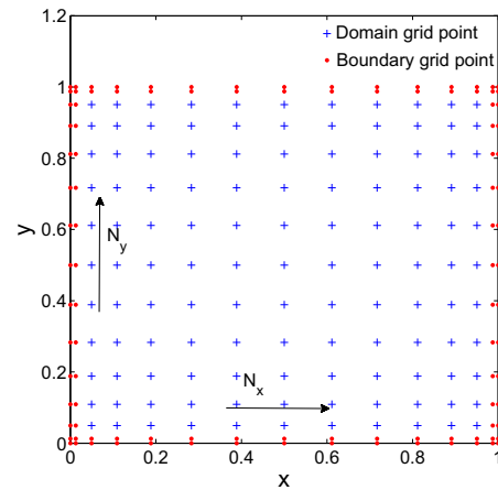
Fig. 1. DQM grid distribution in two-dimension.
