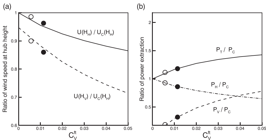
Figure 13. Ratios of (a) wind speeds at the hub heights and (b) plane-averaged unit power extraction from the analytical model as a function of c_{T,V}^{ft} . The lines are model predictions, the open circles are LES results with C_T^V = 0.25 and the filled circles are LES results with C_T^V = 0.50 . The subscript ‘C’ denotes the control wind farm, ‘V’ for ‘VAWT’, ‘H’ for ‘HAWT’ and ‘T’ for ‘total’.
