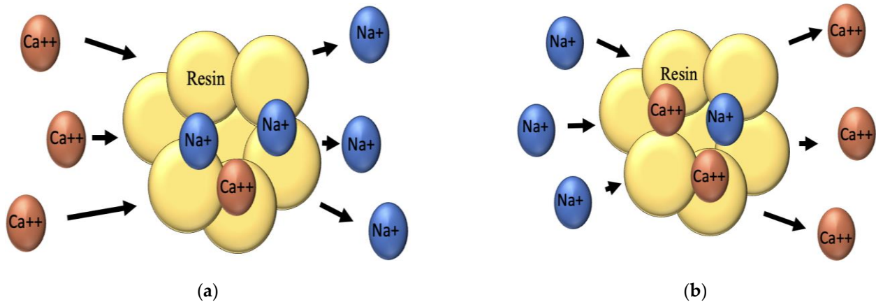
Figure 6. (a) Schematic of the ion-exchange process and (b) resin regeneration.
