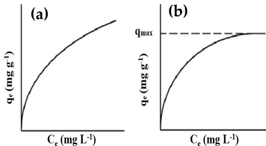
Figure 11. (a) Freundlich adsorption isotherm, and (b) Langmuir adsorption isotherm.
