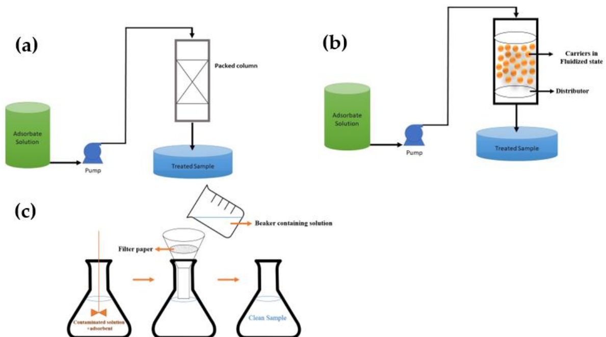
Figure 10. Different configurations for adsorption of impurities: (a) Packed-bed adsorber, (b) Fluidized-bed adsorber, and (c) Batch experiments.
