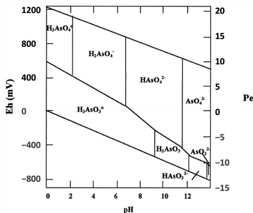
Figure 3. Eh–H diagram for aqueous arsenic species at 25 °C. (reprinted from [15] with Elsevier permission).
