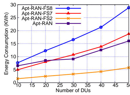
Fig. 21: Total energy consumption (KWh) vs number of DUs for different split options in a day.
