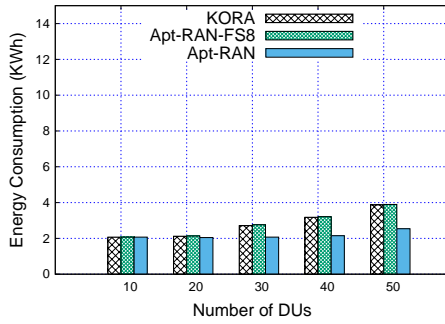
Fig. 11: Total energy consumption (KWh) vs number of DUs during Low_Load (12AM-8AM).
