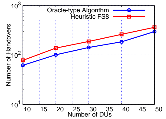
Fig. 30: Comparison between Heuristic FS8 and Oracle-type Algorithm for Total Number of Handovers in a day.
