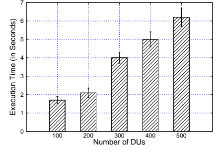
Fig. 25: Run-time performance and scalability of heuristic algorithm.
