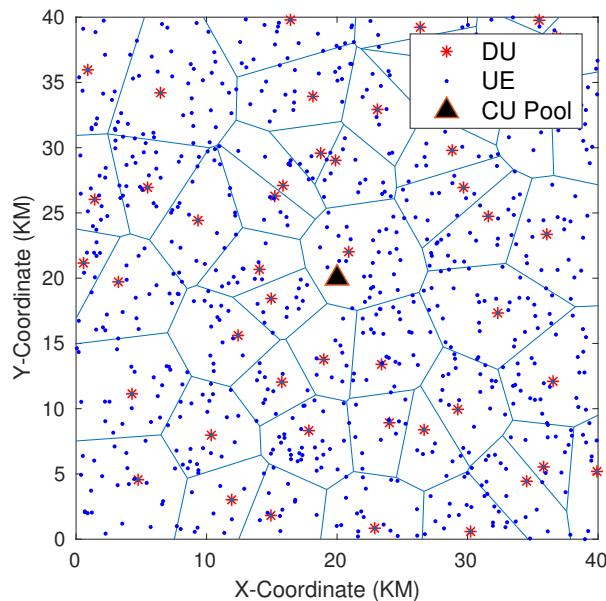
Fig. 7: Spatial distribution of 500 UEs and 50 DUs as per MHCPP II.
