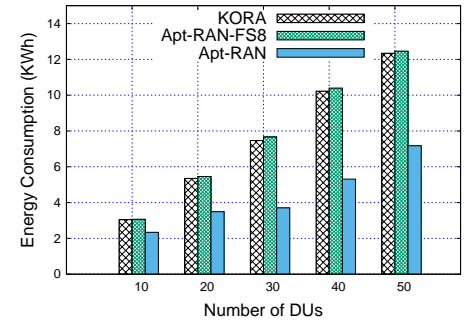
Fig. 13: Total energy consumption (KWh) vs number of DUs during High_Load (12PM-8PM).
