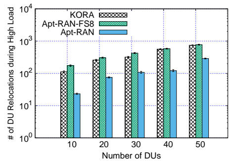
Fig. 16: Total number of DU relocations vs number of DUs during High_Load (12PM-8PM).
