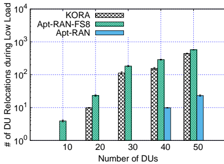
Fig. 14: Total number of DU relocations vs number of DUs during Low_Load (12AM-8AM).
