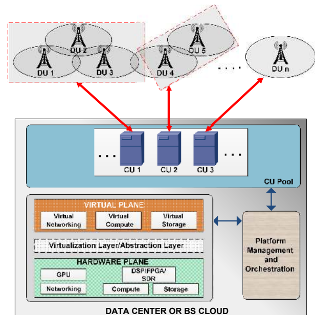
Fig. 1: Programmable & virtualized computing center for CUs in NG-RAN.
