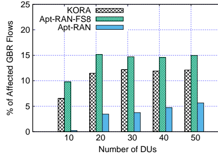
Fig. 18: Percentage of GBR flows affected vs number of DUs during Medium_Load (8AM-12PM & 8PM-12AM).
