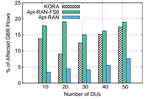
Fig. 19: Percentage of GBR flows affected vs number of DUs during High_Load (12PM-8PM).
