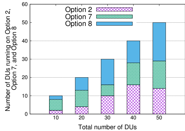
Fig. 10: DUs running on different split options vs total number of DUs.
