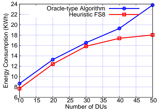
Fig. 29: Comparison between Heuristic FS8 and Oracle-type Algorithm for Total Energy Consumption in a day.
