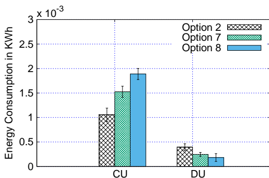
Fig. 5: Energy consumption for 120 seconds for different split options (Option 2, Option 7, and Option 8) at CU and DU.
