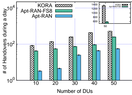
Fig. 20: Total number of handovers vs number of DUs in a day.
