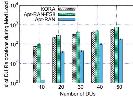
Fig. 15: Total number of DU relocations vs number of DUs during Medium_Load (8AM-12PM & 8PM-12AM).
