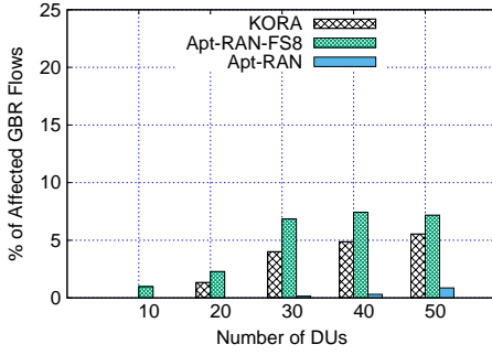
Fig. 17: Percentage of GBR flows affected vs number of DUs during Low_Load (12AM-8AM).
