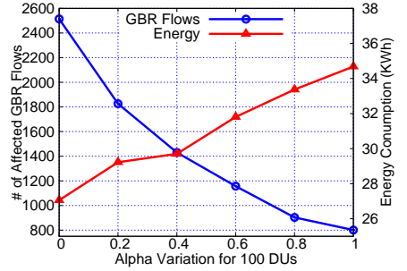
Fig. 28: Effect of \alpha on affected GBR flows and energy consumption in heuristic for 100 DUs.
