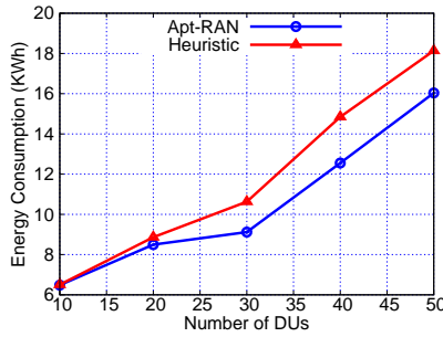
Fig. 23: Total energy consumption vs number of DUs in a day.
