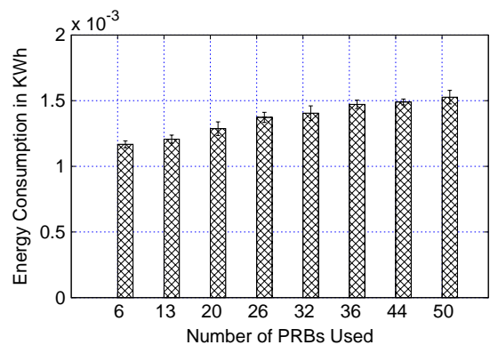
Fig. 6: Variation in energy consumption at CU vs number of PRBs used for 120 seconds for split Option 7.
