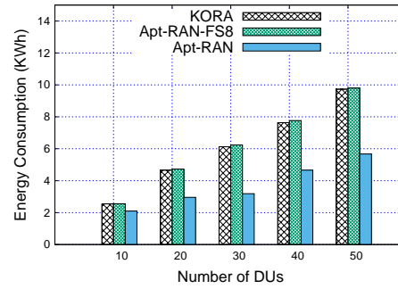
Fig. 12: Total energy consumption (KWh) vs number of DUs during Medium_Load (8AM-12PM & 8PM-12AM).
