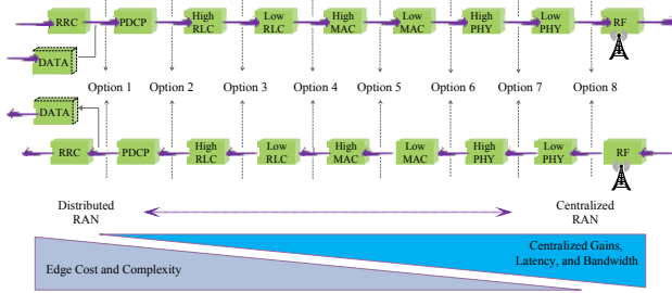
Fig. 3: Split options as defined in 3GPP TR 38.801.
