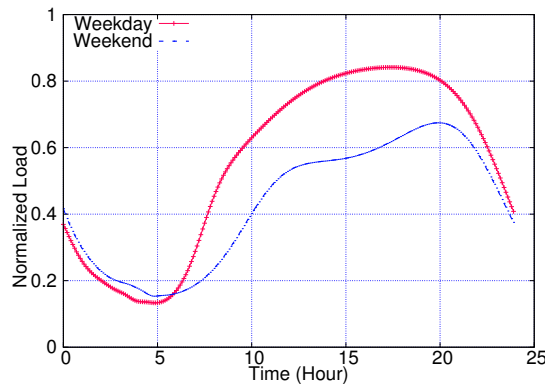
Fig. 2: Time varying normalized mean traffic load at the cell site.
