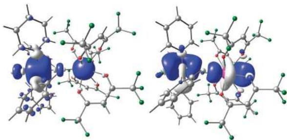
Fig. 4 (left) Spin density plot for the parent Cr–Gd complex. (right) Representation of charge transfer donor(Cr III 3d 2 )–acceptor(Gd III 5d 2 ) NBO plot from second order perturbation theory analysis.
