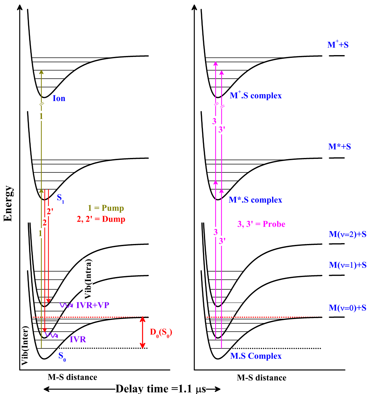
FIG. 1. Schematic level diagram of the SEP-R2PI experiment applied to M\cdot S complex. 9 The potential energy curves indicate the S_0 , S_1 and ion ground-state potentials plotted against the M\cdots S stretching coordinate). The intramolecular vibrational levels of M are indicated by vertically shifted potential curves, drawn for the S_0 state only. The pump/dump steps take place nearly simultaneously, the two-photon ionization probe pulse is applied 1.1 \mu\text{s} later. IVR=intramolecular vibrational redistribution, VP=vibrational predissociation
