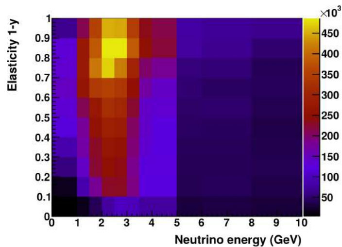
Figure A.8. All neutrino events in the nominal 25 t FV, in FHC at 1.07 MW, per year, rates are per bin. The elasticity is the fraction of the original neutrino energy carried by the outgoing lepton.
