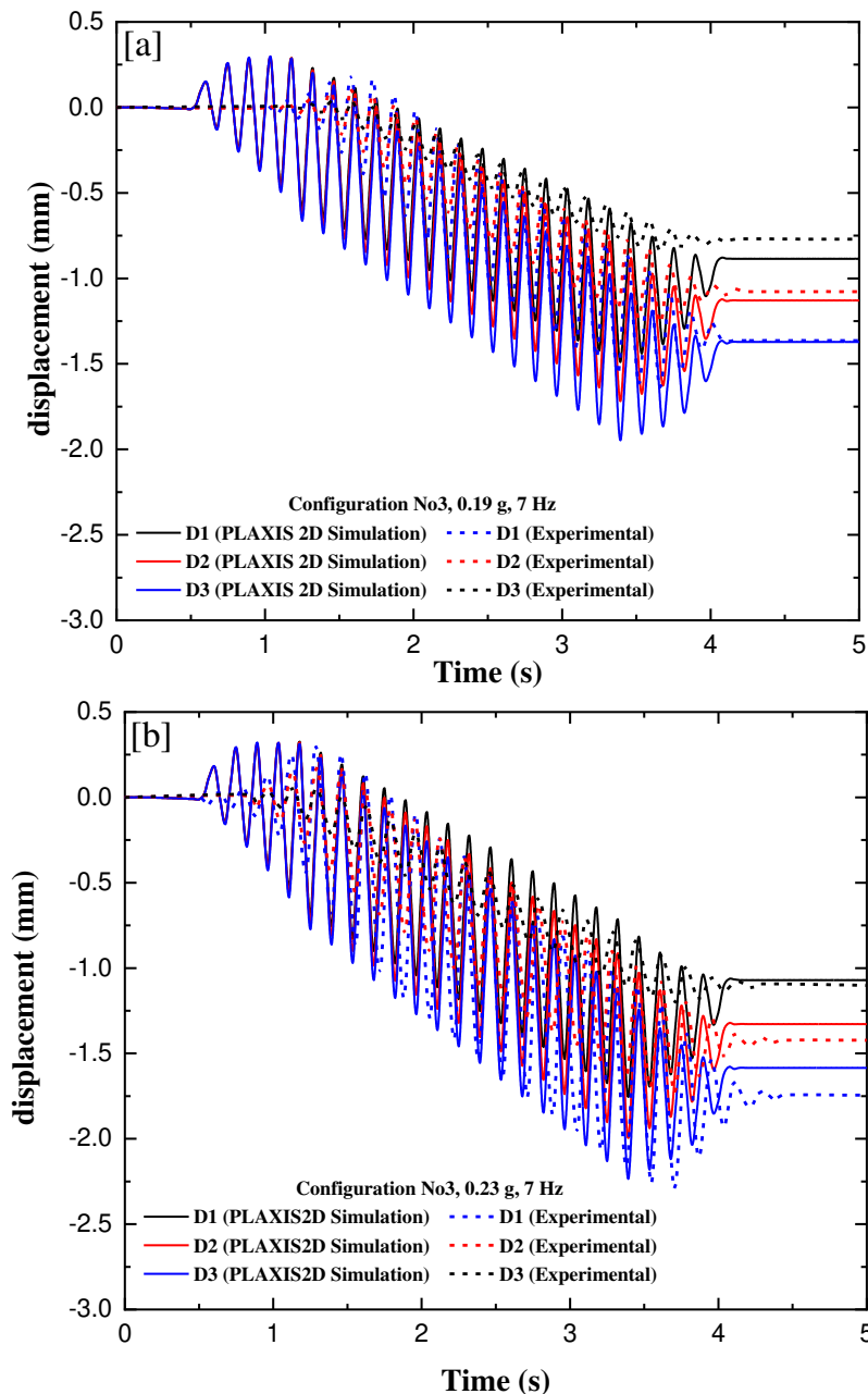
Figure 7. Comparison of results from numerical and physical model tests on Configuration N°3 under sinusoidal-harmonic excitation ( a = 0.19 \text{ g} , 0.23 \text{ g} , and f = 7 \text{ Hz} ): Horizontal displacement time-histories on the cantilever wall stem
