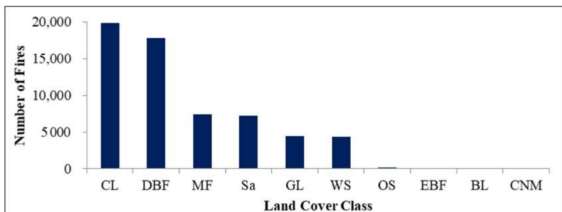
Figure 3. Fires in different land use land cover classes between 2001 and 2021. CL (Cropland), DBF (Deciduous Broadleaf Forest), MF (Mixed Forest), SA (Savannas), GL (Grassland), WS (Woody Savannas), OS (Open Shrubland), EBF (Evergreen Broadleaf Forest), BL (Barren Land), and CNM (Cropland/Natural Vegetation Mosaic).
