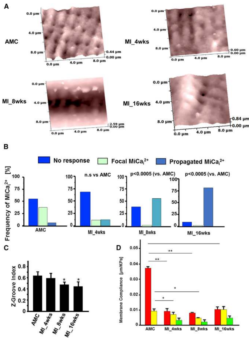
Figure 2. MiCa i Propagation Changes from Local to General during Progression to Heart Failure
