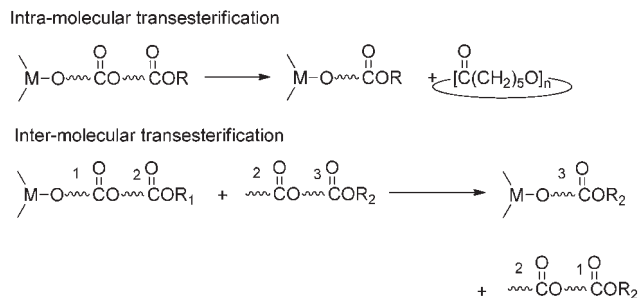
Chart 1 Intramolecular and intermolecular trans-esterification.
