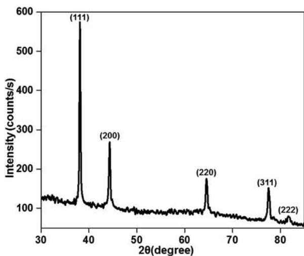
Fig. 3 X-ray diffraction pattern of the plasma-reduced silver nanoparticles (at 16 kV voltage and 300 sccm Ar gas flow).
