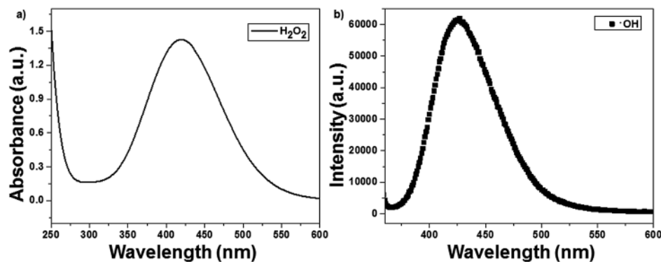
Fig. 8 Identification of reactive oxygen species with 1 wt% Ag(P)-TiO 2 catalyst: (a) H 2 O 2 and (b) ·OH.
