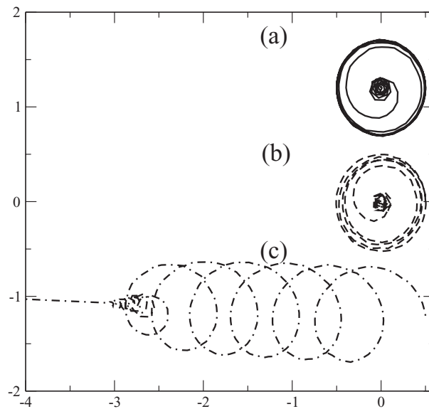
FIG. 9. Trajectory of a single vortex with Re = 10\,000 (a) no stratification, (b) with Boussinesq approximation at Fr = 3 , (c) with only inertial effects of stratification at At = 0.0954 . For visual clarity, the curves are shifted vertically from each other.
