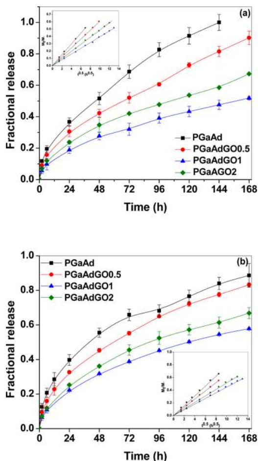
Figure 6. In vitro dye release profiles of PGaAd and composites in 20 mL of PBS solution (pH = 7.4). Release of (a) RB and (b) RBB. The insets of all of the plots show the variation of M_t/M_\infty with t^{0.5} , and the release rate constant, k_{RB} and k_{RBB} , are obtained from the slopes of the linear plot and are tabulated in Table 1.
