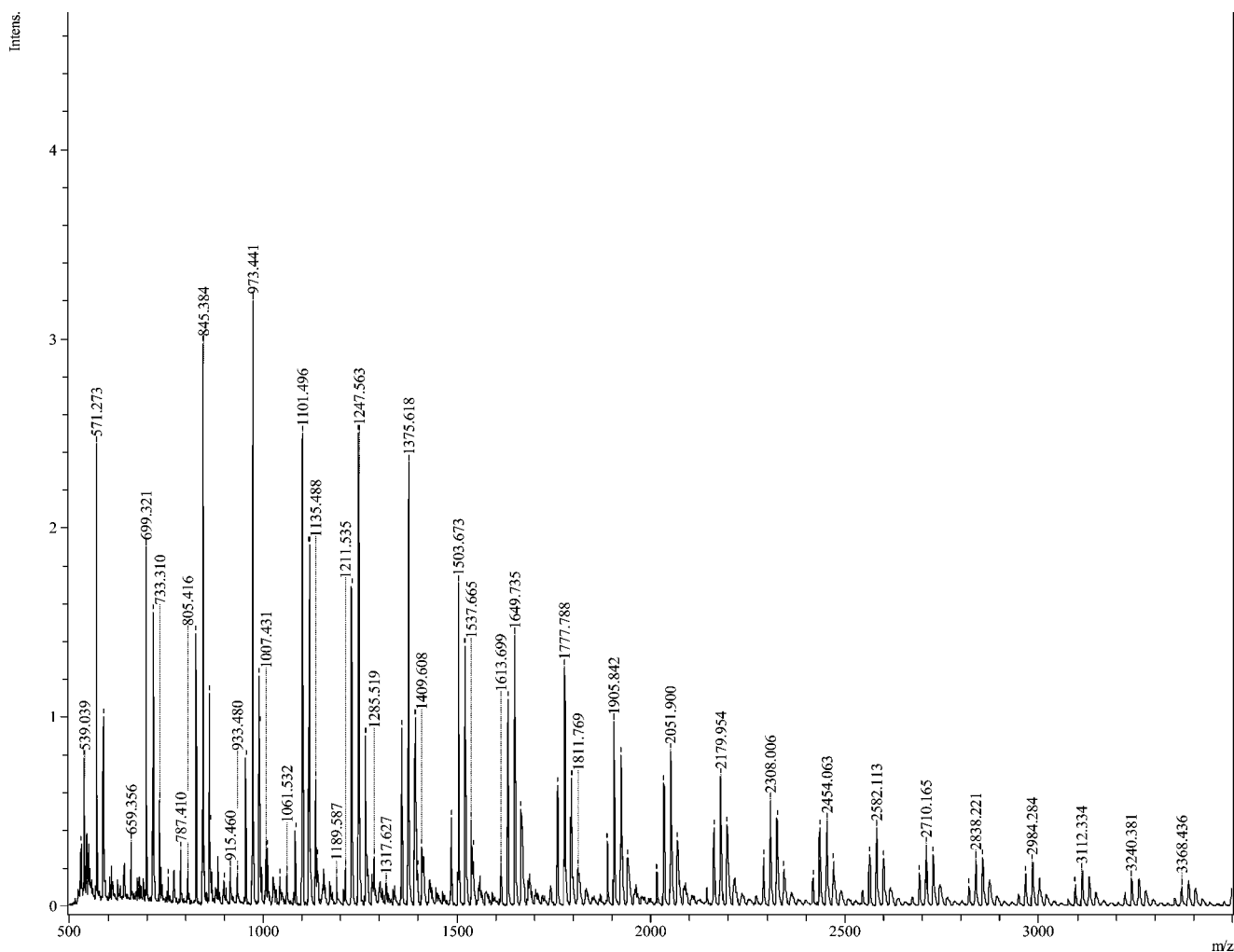
Figure 3. MALDI-TOF MS spectrum of PGaAd.
