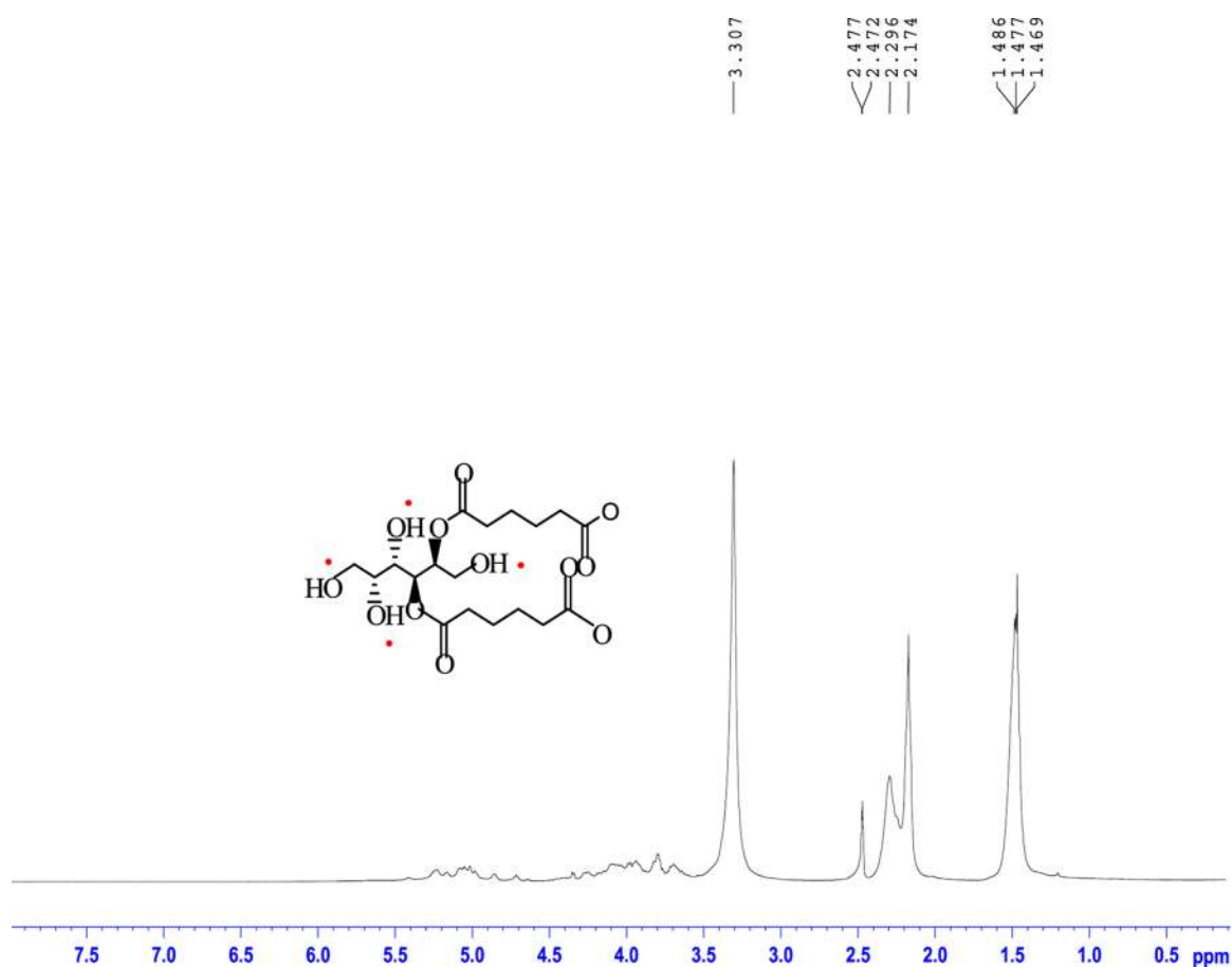
Figure 2. NMR spectra of the prepolymer of PGaAd.
