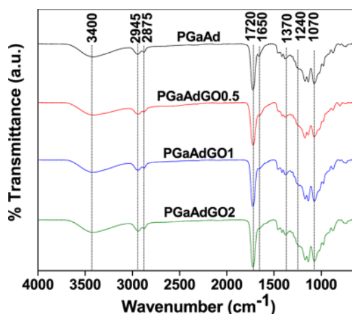
Figure 1. FTIR spectra of PGaAd and composites.
