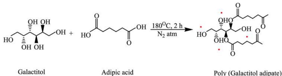
Scheme 1. Plausible Reaction Scheme for the Synthesis of the Galactitol/Adipic Acid Polyester in the Ratio of 1:1 a
