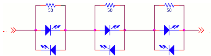
Figure 68. Example schematic for the LED chain, providing failure tolerance and two LED illumination spectra.
