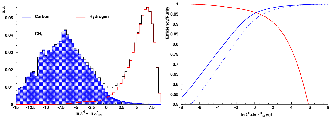
Figure 140. (Left): Example of kinematic identification of \nu(\bar{\nu})\text{H} interactions for the \nu_\mu p \rightarrow \mu^- p \pi^+ CC topologies reconstructed in the STT. The distributions of the logarithm of the likelihood ratio H/C for the H signal, the C background, and the \text{CH}_2 plastic (sum) are shown. (Right): Efficiency (red color) and purity (blue color) as a function of the kinematic cut for the exclusive processes \nu_\mu p \rightarrow \mu^- p \pi^+ (solid lines) and \bar{\nu}_\mu p \rightarrow \mu^+ p \pi^- (dashed-dotted lines) on H [50].
