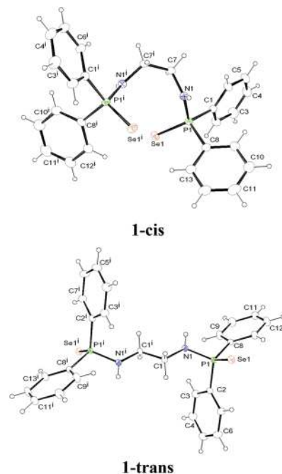
Fig. 1 Solid-state structures of compounds 1-cis and 1-trans , ellipsoids are drawn to encompass 30 per cent probability. Selected bond lengths [Å] and bond angles [°]: 1-cis : P1–N1 1.665(2), P1–Se1 2.1194(7), P1–C1 1.810(3), P1–C8 1.810(3), N1–C7 1.468(3), C7–C7 i 1.512(5), C7 i –C7–N1 112.9(2), N1–P1–C8 102.55(12), N1–P1–Se1 116.97(8), N1–P1–C1 104.95(12), P1–N1–C7 120.73(18), Se1–P1–C8 113.29(10), Se1–P1–C1 111.36(9). 1-trans : P1–N1 1.6660(18), P1–Se1 2.1057(5), P1–C2 1.817(2), P1–C8 1.816(2), N1–C1 1.468(3), C1–C1 i 1.507(4), C1 i –C1–N1 109.4(2), N1–P1–C8 101.65(9), N1–P1–Se1 118.10(7), N1–P1–C2 102.72(10), P1–N1–C1 117.58(14), Se1–P1–C8 112.19(7), Se1–P1–C2 112.45(7).
