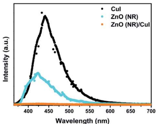
Fig. 3 Photoluminescence spectra of ZnO nanorods, CuI and ZnO/CuI.
