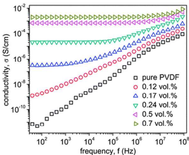
Figure 3: Conductivity plot of PVDF with various vol.% of TRG-PVDF (He et al. 38 Reproduced by the permission of The Royal Society of Chemistry)
