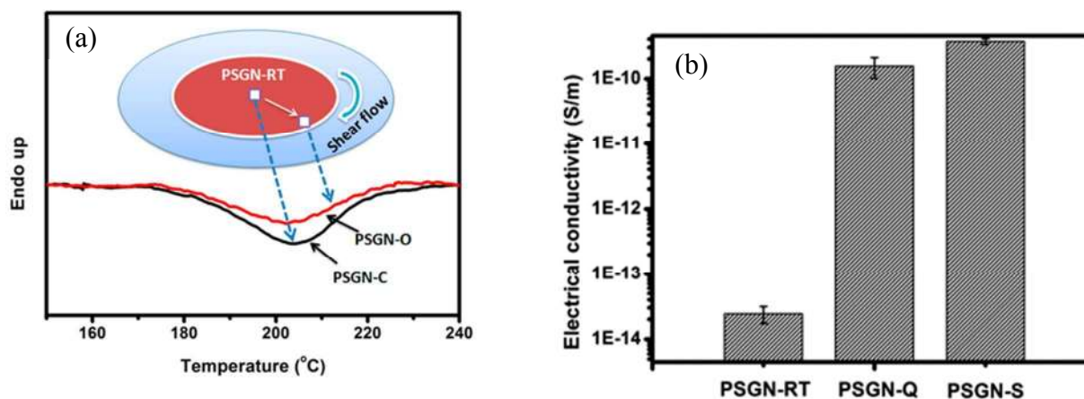
Figure 10: Shows (a) schematic of DSC scans of GO in various zones (b) exhibits conductivity of neat polystyrene composite, quiescent and sheared polystyrene composite (Ye et al. 45
