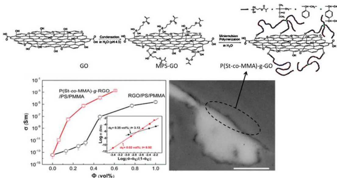
Figure 9: Schematic of covalent functionalization of GO and Conductivity plot of PS/PMMA blend with rGO and P(St-co-MMA) copolymer grafted GO. (Tan et al. 48 Reproduced by the permission of The Royal Society of Chemistry)
