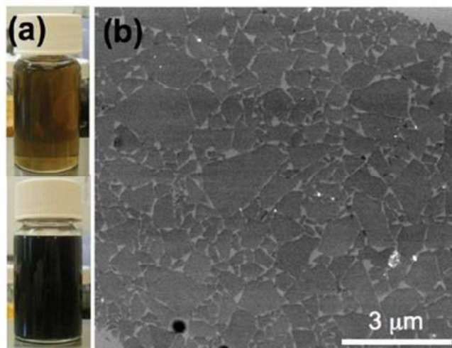
Figure 6: (a) Optical images of a graphene oxide suspension in PC (top) before and (bottom) after heating at 150 °C for 12 h. (b) SEM image of graphene oxide platelets deposited on a Si substrate. (Zhu et al. 42 Reproduced by permission of American Chemical Society Copyright © 2010, American Chemical Society)
