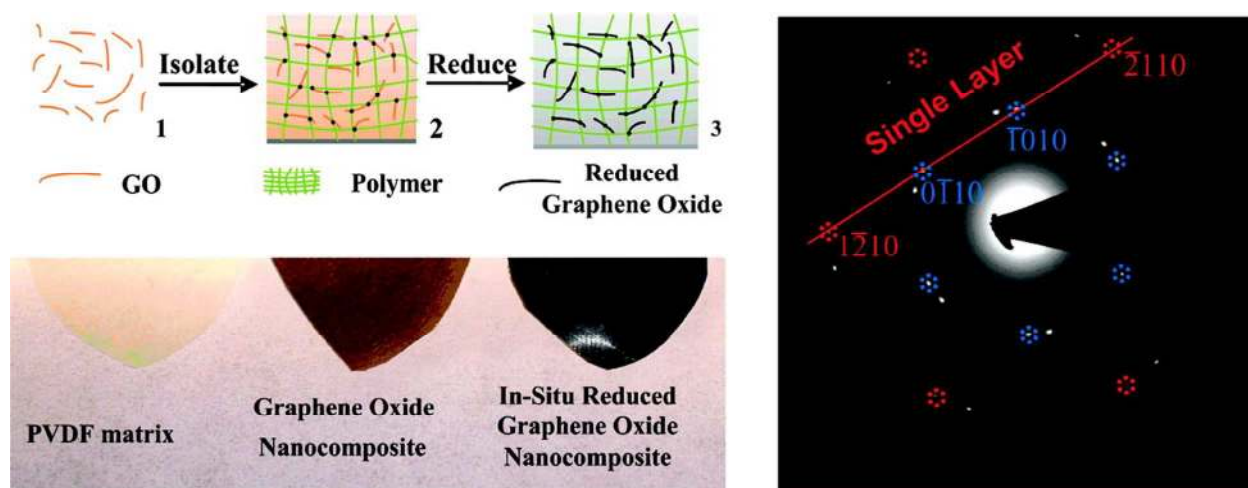
Figure 2: In situ reduction during compositing process (Tang et al. 37 Reproduced by permission of American Chemical Society Copyright © 2012, American Chemical Society)
