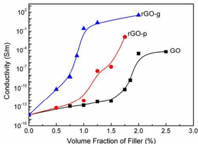
Figure 5: Plots of electrical conductivity versus filler loading for PLA composites (Shen et al. 41 Reproduced by permission of Elsevier, Copyright © 2012 Elsevier Ltd.)
