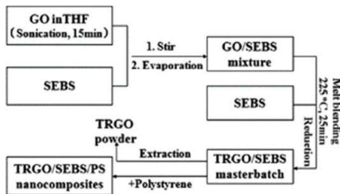
Figure 11: In situ reduction of GO via mater batch in polystyrene (You et al. 49 Reproduced by
