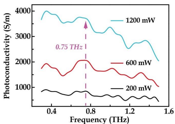
Figure S3. Numerically extracted photoconductivity values as a function of frequency at a selection of average optical pump powers.
