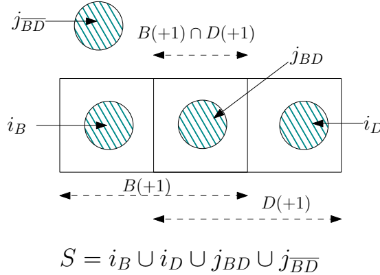
Fig. 1. S is some r -sized subset of [n] . Let i_B = S \cap (B(+1) \setminus D(+1)) , i_D = S \cap (D(+1) \setminus B(+1)) , j_{BD} = S \cap (B(+1) \cap D(+1)) and j_{\overline{BD}} = S \cap ([n] \setminus (B(+1) \cup D(+1))) . So, S = i_B \cup i_D \cup j_{BD} \cup j_{\overline{BD}} . If S is an unbiased representative for B , then |i_B| + |j_{BD}| = |i_D| + |j_{\overline{BD}}| . If S is an unbiased representative of D , then |i_D| + |j_{BD}| = |i_B| + |j_{\overline{BD}}| . So, if S is an unbiased representative of both B and D , then |i_B| = |i_D| and |j_{BD}| = |j_{\overline{BD}}| .
